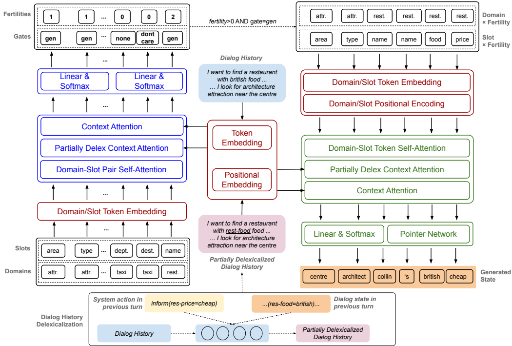
Figure 1: Our NADST has 3 key components: encoders (“red”), fertility decoder (“blue”), and state decoder (“green”). (i) Encoders encode sequences of dialogue history, delexicalized dialogue history, and domain and slot tokens into continuous representations; (ii) Fertility Decoder has 3 attention mechanisms to learn potential dependencies across ( domain , slot ) pairs in combination with dialogue history. The output is used to generate fertilities and slot gates; and (iii) State Decoder receives the input sequence including sub-sequences of ( domain , slot ) \times fertility to decode a complete dialogue state sequence as concatenation of component slot values. For simplicity, we do not show feedforward, residual connection, and layer-normalization layers in the figure. Best viewed in color.
