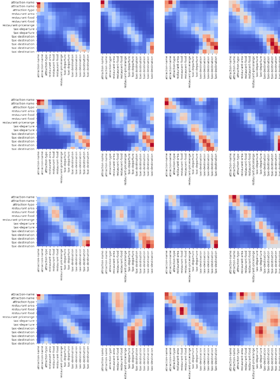
Figure 6: Visualization of all attention heads in the last attention step T_{state} in the state decoder. The DST prediction is done for the 6 th turn in dialogue ID PMUL3759 in MultiWOZ2.1.
