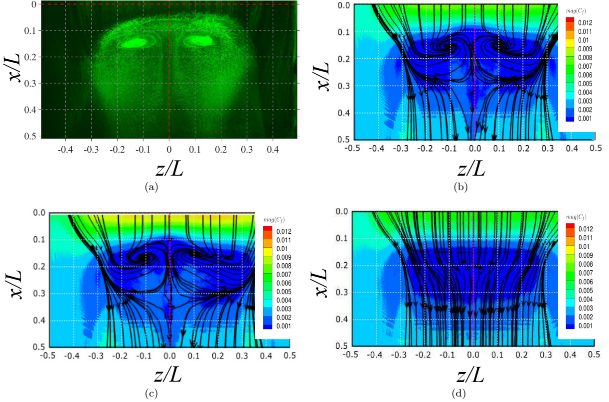
FIG. 18. (a) An oil-flow visualization of the counter-rotating vortices in the region of separation (as observed experimentally [62]); reprinted with permission of the American Institute of Aeronautics and Astronautics, Inc. In sub-plots (b), (c) and (d) we compare the surface streamlines in the separation region for DSM, DTCSM and Vreman models respectively. It is also noticeable that for DTCSM, the skin friction at the apex of the bump is inline with the experimental value (from Figure 15) and higher than DSM and Vreman models.
