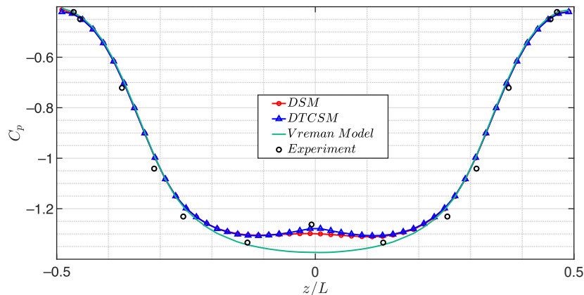
FIG. 17. Spanwise distribution of the surface pressure coefficient for the three dimensional bump at Re_L = 3.41 \times 10^6 for DSM, DTCSM and Vreman model for the fine mesh case. The black dots represent the experiments of Williams et al. [62].
