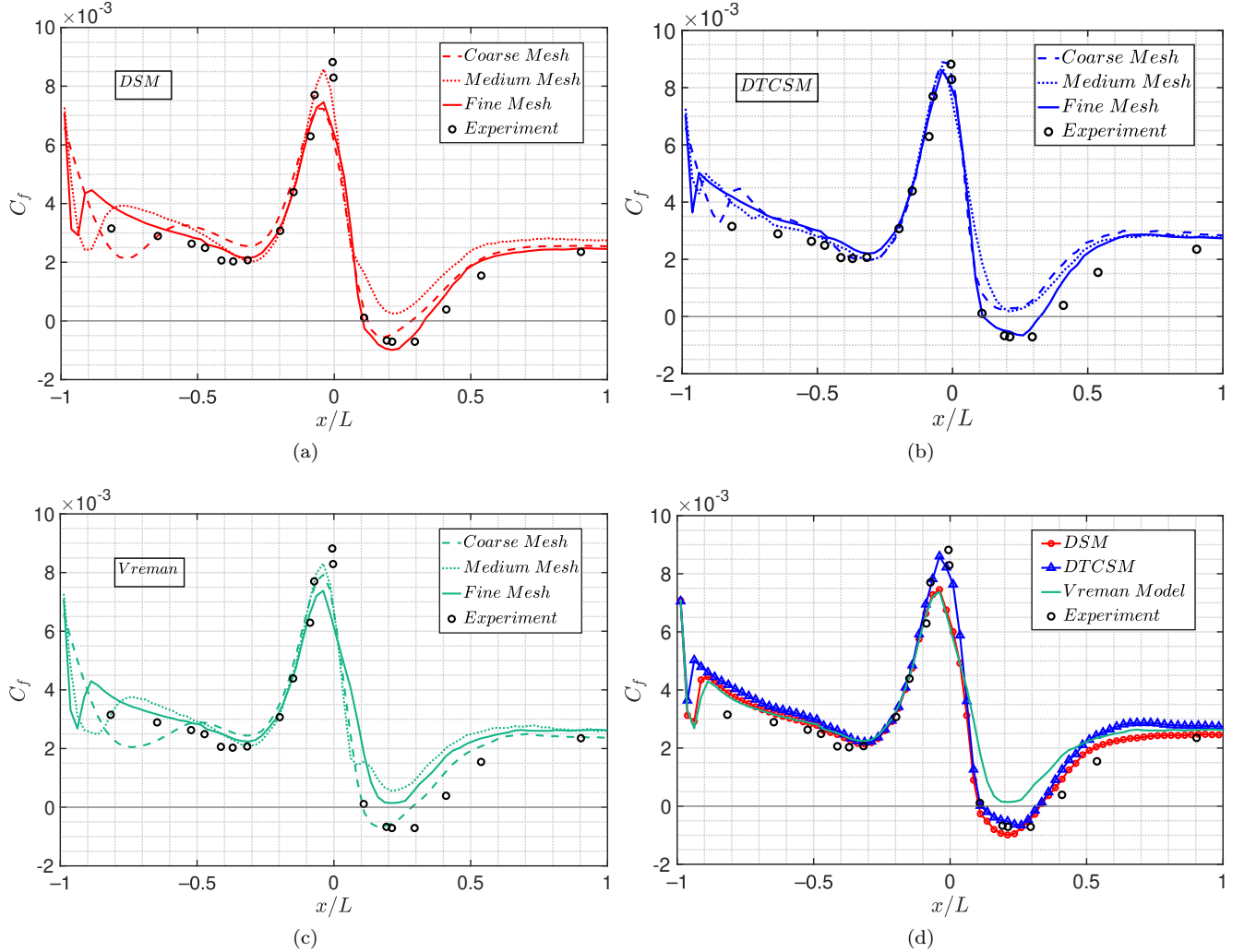
FIG. 15. Streamwise distribution of the mid-span surface friction coefficient for the three dimensional bump at Re_L = 3.41 \times 10^6 for (a) DSM, (b) DTCSM and (c) Vreman model. The equilibrium wall model is applied and three mesh resolutions are shown. Finally, sub-plot (d) compares the prediction of C_f by the three models on the fine mesh. The black dots represent the experiments performed by Gray et al. [24].
