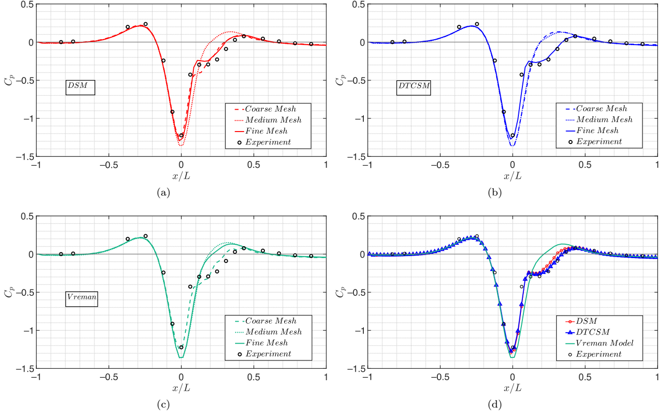
FIG. 16. Streamwise distribution of the mid-span surface pressure coefficient for the three dimensional bump at Re_L = 3.41 \times 10^6 for (a) DSM, (b) DTCSM and (c) Vreman model. Finally, sub-plot (d) provides a comparison of the three models for the fine mesh. The black dots represent the experimental measurements of Williams et al. [62].
