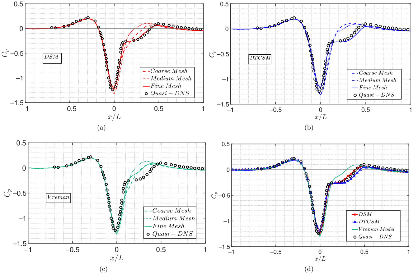
FIG. 14. Streamwise distribution of the surface pressure coefficient for the spanwise-periodic bump at Re_L = 2 \times 10^6 for (a) DSM, (b) DTCSM and (c) Vreman Model. The equilibrium wall model is applied and three mesh resolutions are shown. Finally, sub-figure (d) provides a comparison of the three SGS models for the fine mesh. The black symbols represent the quasi-DNS of Uzun and Malik [56].
