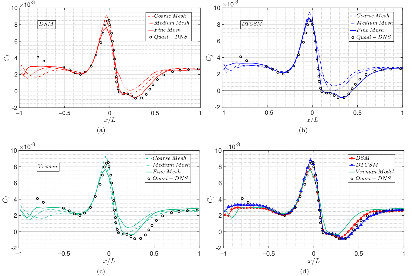
FIG. 13. Streamwise distribution of the surface friction coefficient for the spanwise-periodic bump at Re_L = 2 \times 10^6 for (a) DSM, (b) DTCSM and (c) Vreman Model. The equilibrium wall model is applied and three mesh resolutions are shown. Finally, sub-figure (d) provides a comparison of the three SGS models for the fine mesh. The black symbols represent the quasi-DNS of Uzun and Malik [56].
