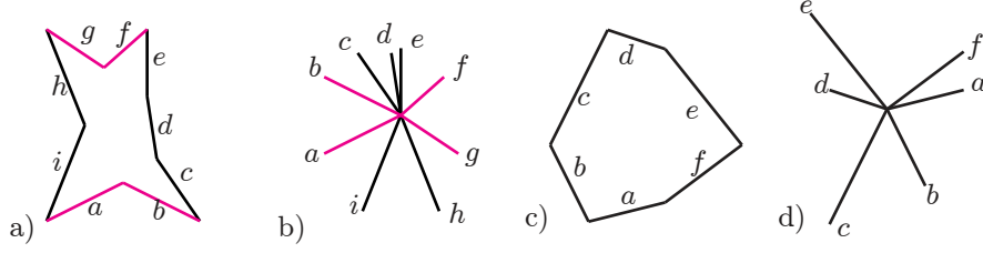
FIGURE 12. A pseudo-quadrangle with all angles face-proper (a) and a convex face with no sign changes (c), with dual vertices. Line weights indicate stress signs.
