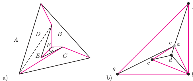
FIGURE 19. A pseudo-triangulation with two non-pointed vertices (b) with its reciprocal (a), a singular pseudo-triangulation.
