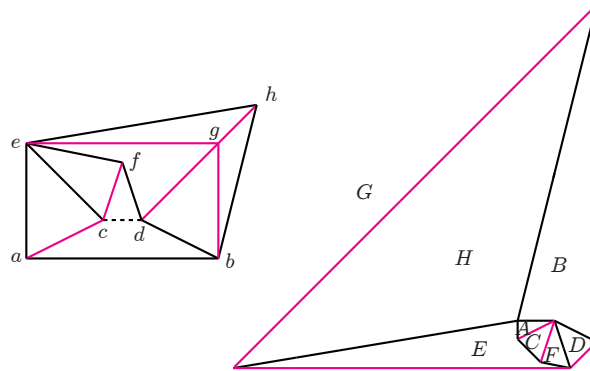
FIGURE 23. A pseudo-quadrangulation with a good self-stress for which the added edge (dashed) makes a good self-stress on all edges impossible.
