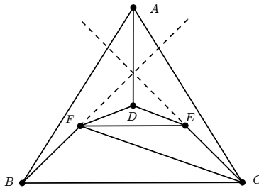
FIGURE 8. A Laman circuit with a singular self-stress.
