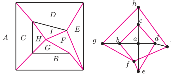
FIGURE 22. The same graph and combinatorial pseudo-quadrangulation can be bad, because of an altered sign pattern.
