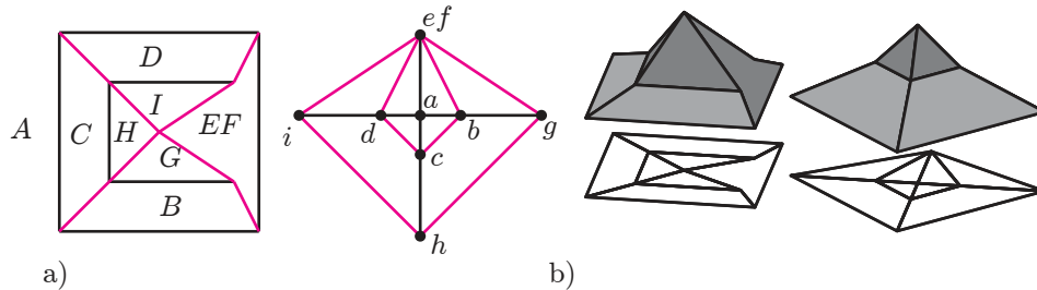
FIGURE 21. A nearby singular framework with its compressed reciprocal and lift.
