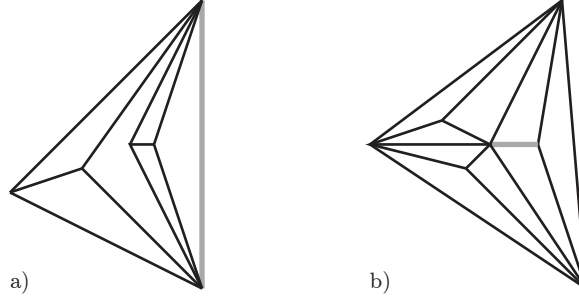
FIGURE 14. These pseudo-triangulations have a self-stress fulfilling all face conditions but do not have a good self-stress.
