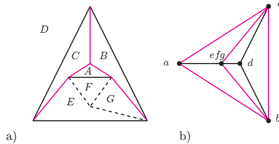
FIGURE 17. A singular stress on a Laman circuit can drop both vertices and edges.
