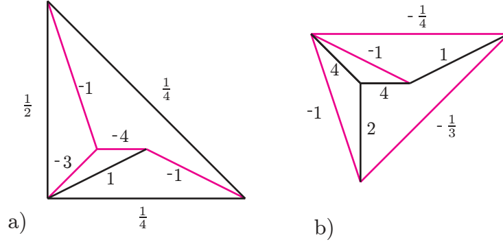
FIGURE 15. A reciprocal pair of Laman circuit pseudo-triangulations.
