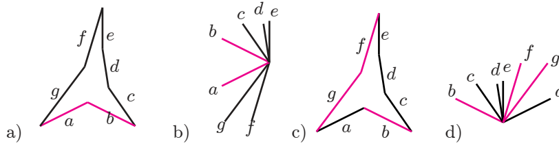
FIGURE 11. (a) a pseudo-triangle with one vertex-proper angle, at the corner between e and f and (b) its reciprocal vertex, (c) a pseudo-triangle with one vertex-proper angle between a and b , not at a corner, and (d) its reciprocal vertex. Stress signs are indicated by line weights.
