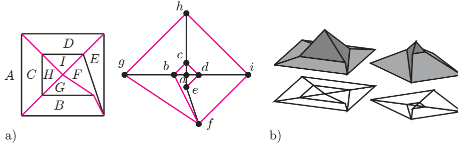
FIGURE 20. A reciprocal pair of pseudo-quadrangulations on a Laman circuit.
