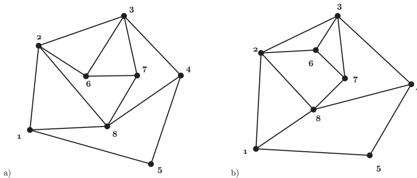
FIGURE 5. (a) A pointed pseudo-triangulation (b) a different embedding of the same graph which is not a pseudo-triangulation.
