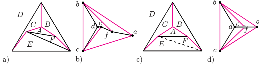
FIGURE 16. A singular self-stress on a Laman circuit pseudo-triangulation can drop an edge from the original graph - and fuse two vertices in the reciprocal.
