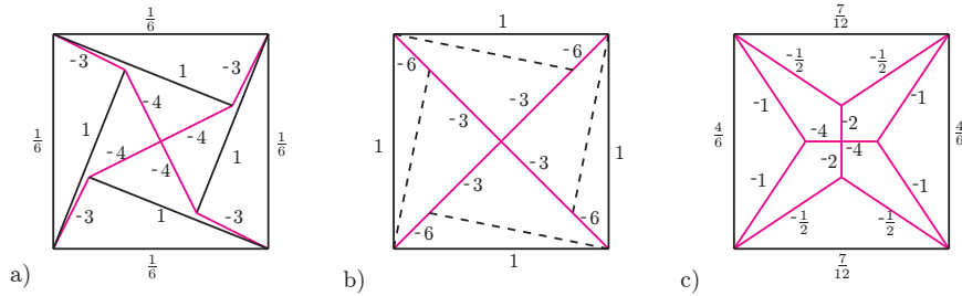
FIGURE 7. A geometric circuit (a), a singular realization with dropped edges (b) and a singular realization with additional self-stresses (c).
