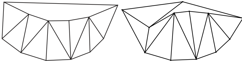
FIGURE 6. A Laman circuit and one of its embeddings as a pseudo-triangulation with exactly one non-pointed vertex.
