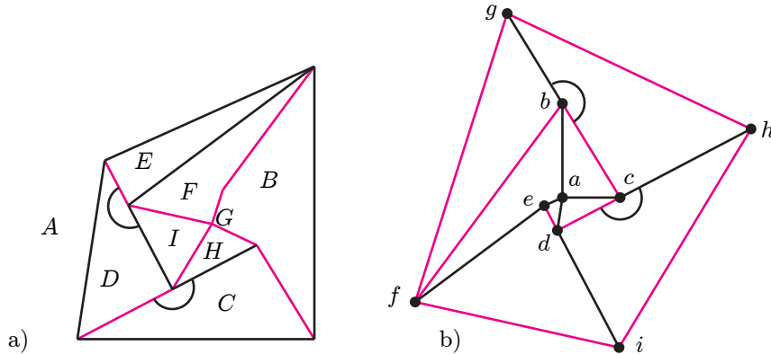
FIGURE 9. We can have flat angles on both sides of a non-crossing reciprocal pair.
