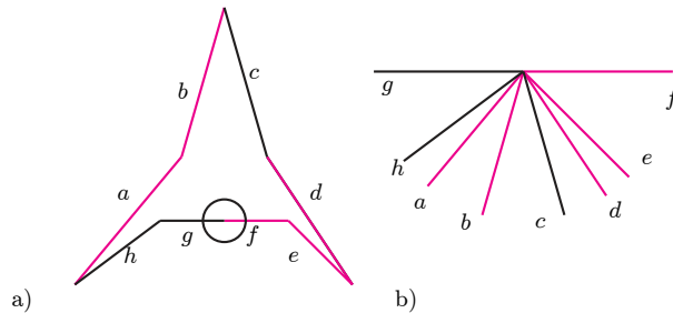
FIGURE 10. Locally, the reciprocal of a pseudo-quadrangle with a flat vertex as a corner is a flat vertex.
