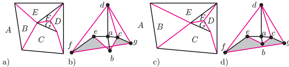
FIGURE 13. Sign conditions are not enough to guarantee a non-crossing reciprocal. The geometric circuit in part (a) has the same signs (and big/small angles) as the one in part (c), but the former produces a crossing reciprocal while the latter produces a non-crossing one.
