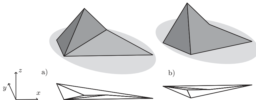
FIGURE 4. The lift of the frameworks of Figure 3.
