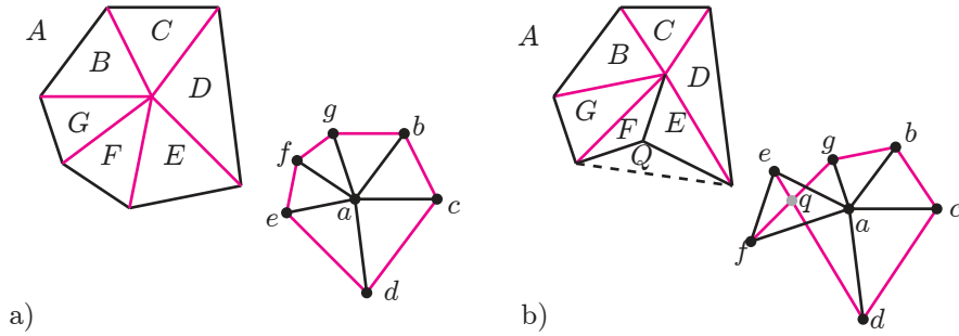
FIGURE 18. Possible pyramids which might be created by a cut near a maximum in the lifting of a non-crossing framework (shown in vertical projection), with their reciprocals.
