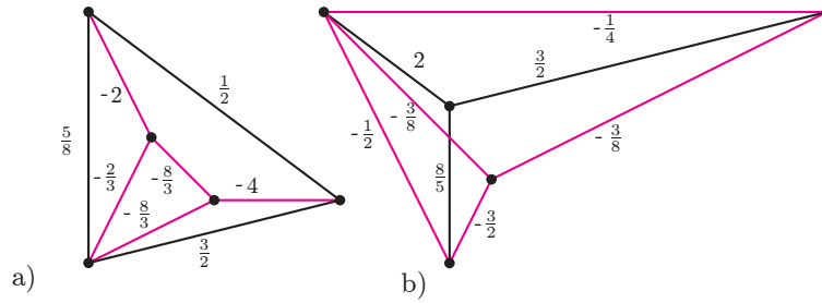
FIGURE 1. A non-crossing framework with crossing reciprocal.
