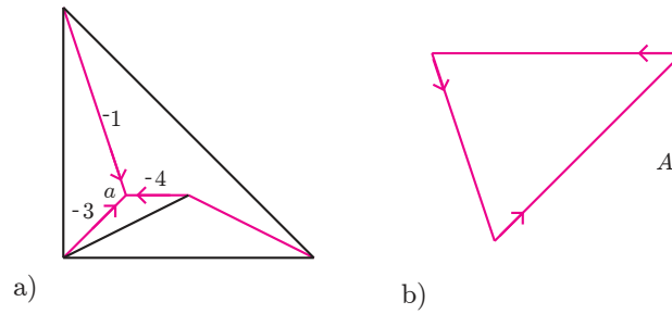
FIGURE 2. The equilibrium forces at vertex a produce a polygon of forces A .
