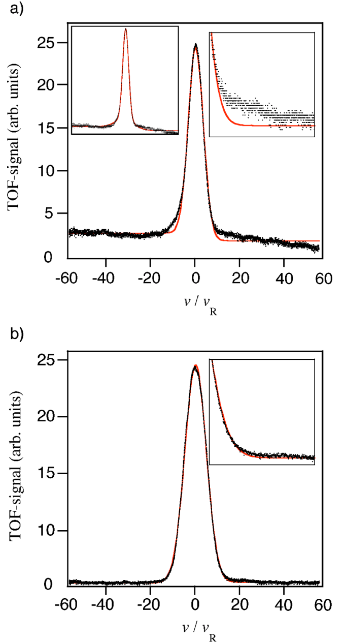
FIG. 3. (Color online) Experimentally recorded velocity distributions with fits to simple Gaussians. These data are recorded with an equilibration time of 25 ms. For (a) the modulation depth of the optical potential was U_0 = 78E_R and the shown data are an average of 20 TOF measurements. For (b) the corresponding facts were U_0 = 285E_R and an average of five TOF measurements. The insets in the top right corners show magnifications of portions of the wings of the distributions. The inset in the top left corner of (a) show the same data with a fit to a double Gaussian.
