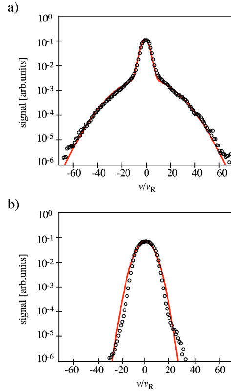
FIG. 11. (Color online) Numerically computed velocity distribution for (a) U_0=78E_R and (b) U_0=293E_R together with fits to double Gaussians.
