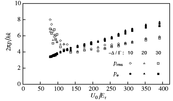
FIG. 8. Comparison between the rms momentum and the width at 1/\sqrt{e} of the momentum distribution as a function of the potential depth U_0 for three different detunings \Delta = -10\Gamma, -20\Gamma, -30\Gamma .
