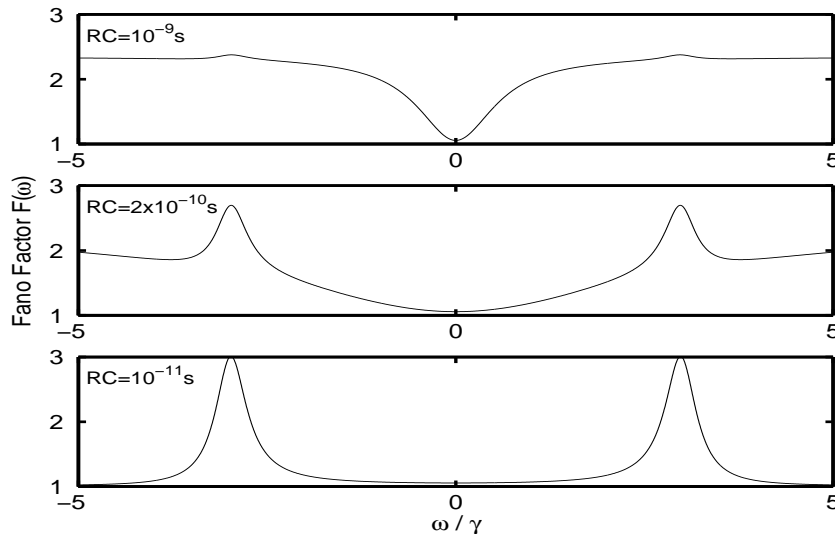
Figure 3. Fano Factor plot for non-ideal measurement of the current when the coupling between the qubit dots is relatively strong: \Omega = 3\gamma . The values of R_i C are given in the plots.
