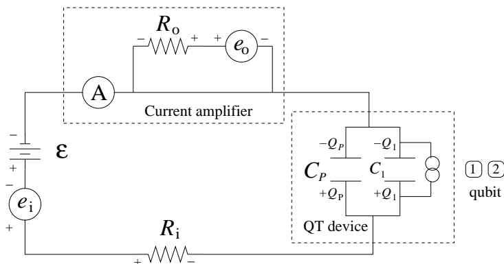
Figure 1. Equivalent circuit for measurement of current through the QT device. The single tunnel junction in the QT device is modelled as a capacitance C_1 . A parasitic capacitance, C_P , between the source and drain is included in parallel with the QT device. Tunnelling events through the device are modelled as a current source.
