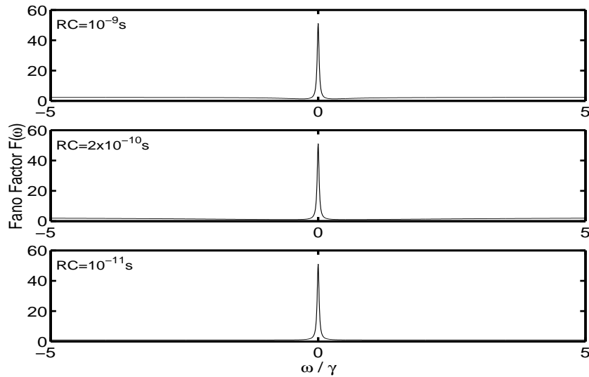
Figure 4. Fano Factor plot for non-ideal measurement of the current when the coupling rate between the qubit dots is an intermediate value: \Omega = 0.6\gamma . The values of R_i C are given in the plots.
