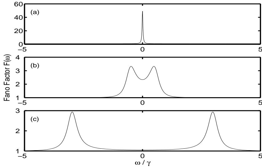
Figure 2. Fano Factor plots for ideal measurement of the current for different values of the tunnel coupling between qubit dots: (a) \Omega = 0.1\gamma , (b) \Omega = 0.6\gamma , (c) \Omega = 3\gamma .
