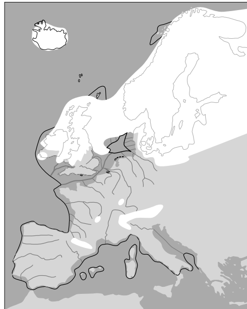
Fig. 4. Topography of NW Europe during the maximum of the Weichselian glaciation (18,000 years B.P.). After Valentin (1957) and Siebert (2001).
