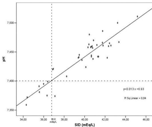
Correlation between the SID and pH (patients with normal UI and PaCO 2 ).
