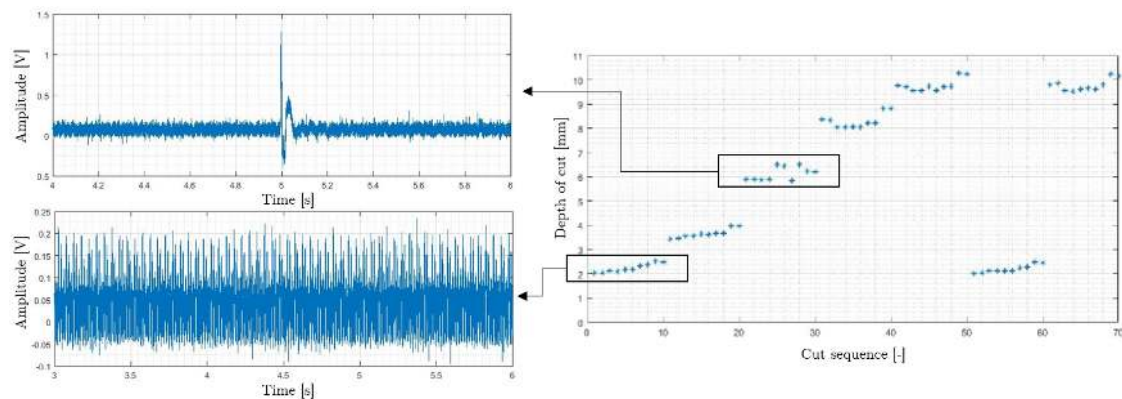
Figure 10. Effect of impacts and high level of background noise on the experimental results.
