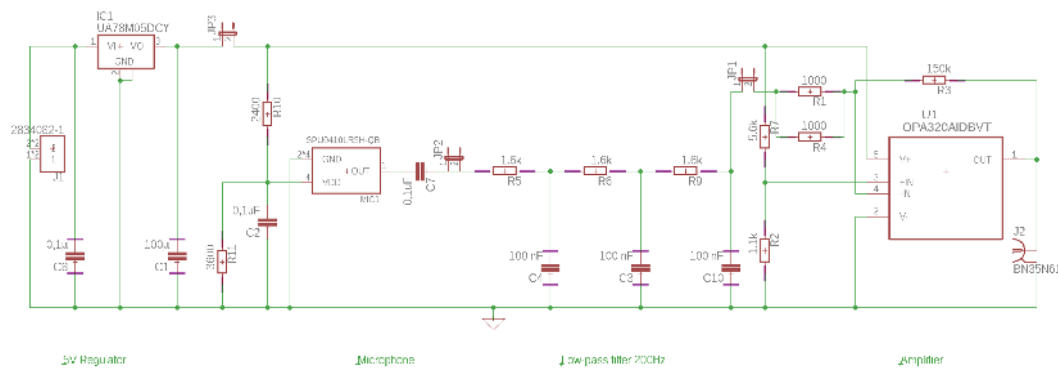
Figure 4. Schematic representation of the conditioning board.
