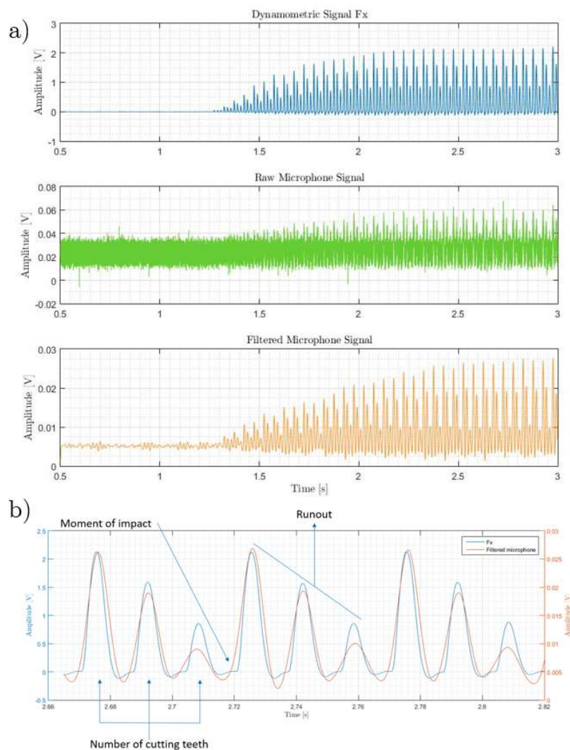
Figure 8. Experimental signals under analysis. (a) Cutting force signal (top), raw AE signal (middle), and filtered AE signal (bottom). (b) Zoomed section of the cutting force and filtered AE signals within the zone of uniform cut.
