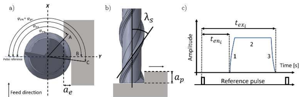
Figure 1. Main parameters of the end-milling process. (a) Top view, (b) front view, and (c) time history of the cutting process.
