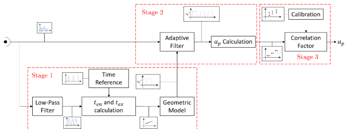
Figure 5. Block diagram of the system.
