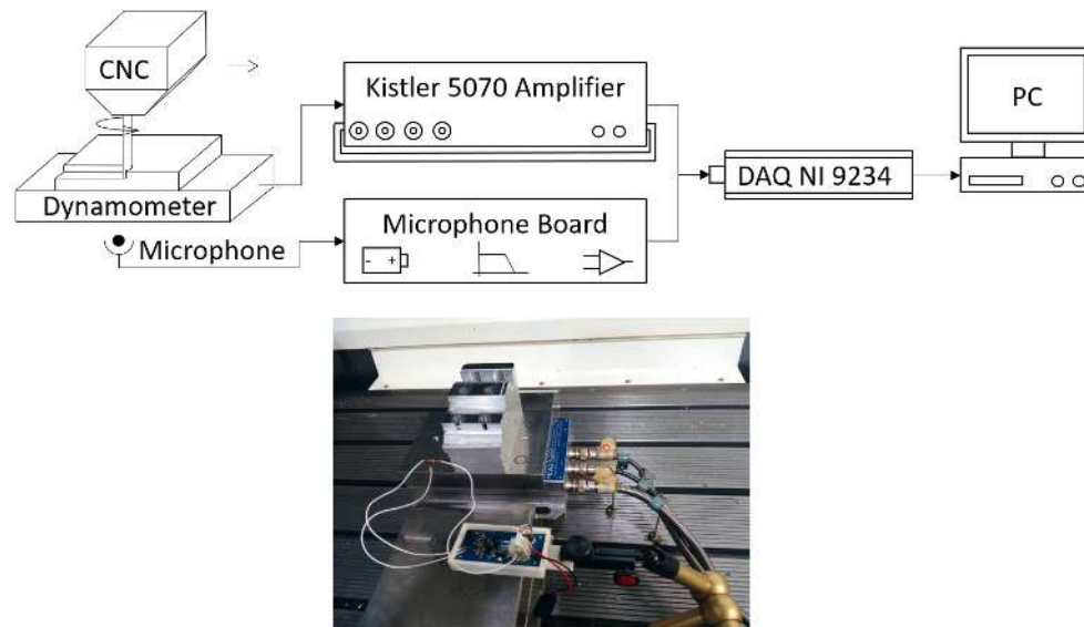
Figure 7. Scheme of the setup (top) and image of the sensors and the piece being machined (bottom).
