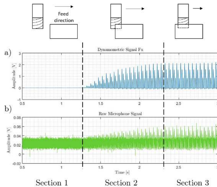
Figure 2. Phases of the end-milling process. (a) Cutting force signal, and (b) acoustic emission (AE) signal.
