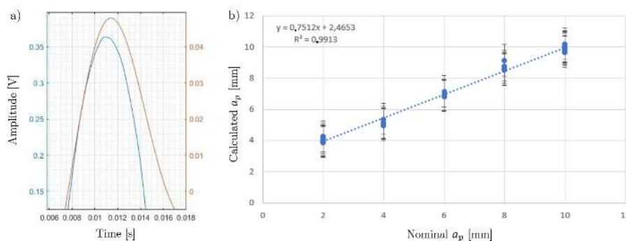
Figure 9. Experimental results. (a) Exit time delay between the cutting force signal (blue) and filtered AE signal (orange). (b) Calibration curve: estimated vs. nominal depth of cut.
