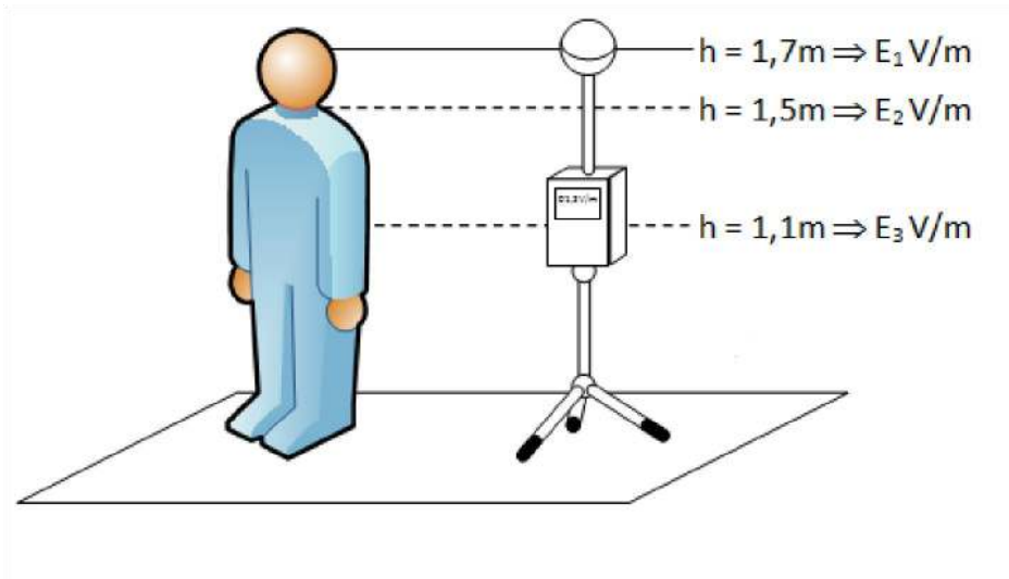
Fig. 4. Illustration of measurements for spatial average determination (adapted from [4]).
