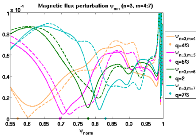
FIG. 51: Radial profile of the Fourier harmonics of the magnetic perturbation |\psi_{m,n}| , m = 4 - 7 in both cases: without diamagnetic effects (dash) and with diamagnetic effects included (full line). The approximate position of the resonant surfaces q = m/n are represented by the dots. All the central harmonics m = 4 - 7 are screened near their corresponding resonant surfaces in both cases
