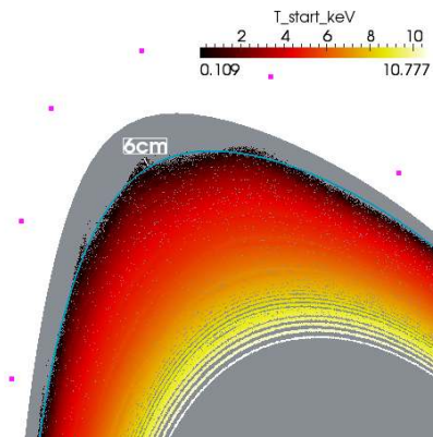
FIG. 38: Magnetic topology at the top of the machine. Small deformations of the separatrix ( \sim 6\text{cm} ) are observed.
