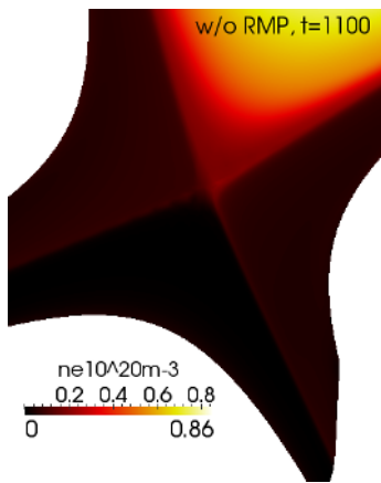
FIG. 42: Density near the X-point without RMPs
