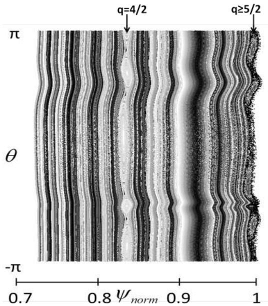
FIG. 14: Poincaré plot of the magnetic topology in (\psi, \theta) coordinates at larger diamagnetic rotation \tau_{IC} = 2 \times 10^{-3} (Resistivity is kept \eta_0 = 10^{-7} ). Note that the islands generated by the RMPs are smaller compared to Fig.13, which points out the larger screening induced by the large diamagnetic (poloidal) rotation.
