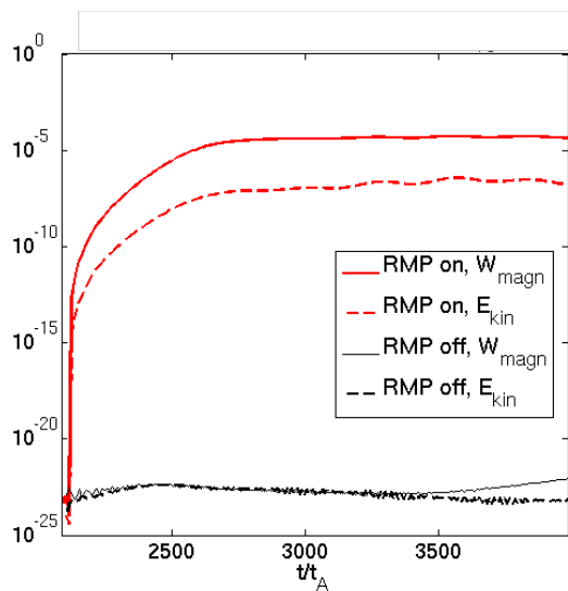
FIG. 10: Magnetic and kinetic energy of the mode n = 2 without/with RMPs, at high resistivity \eta_0 = 10^{-7} and slow diamagnetic rotation ( \tau_{IC} = 10^{-3} )
