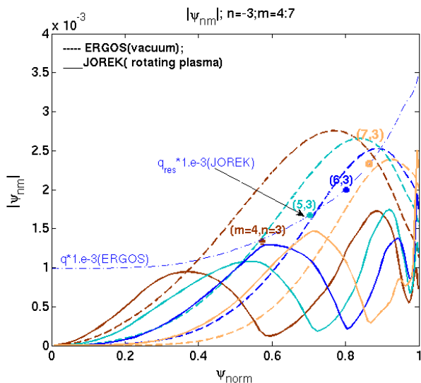
FIG. 34: Fourier harmonics of the magnetic flux perturbation |\psi_{m,n}| , n=3 , m=4-7 in the vacuum case (ERGOS code, dash) and taking into account the plasma response (JOREK, full line). The q -profile is given and the positions of the resonant surfaces are indicated by the dots. Note that compared to the vacuum case, all these harmonics m=4-7 are screened on the corresponding resonant surfaces q=m/n in presence of the rotating plasma.
