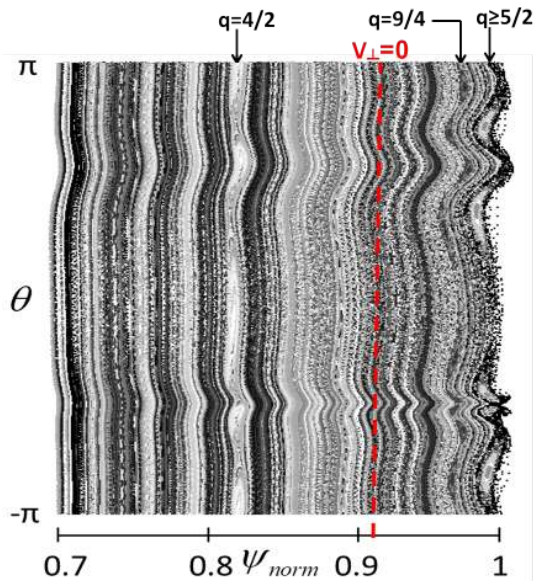
FIG. 22: Poincaré plot of the magnetic topology in (\psi, \theta) coordinates with diamagnetic rotation ( \tau_{IC} = 2 \times 10^{-3} ), parallel source of rotation and neoclassical friction (resistivity \eta_0 = 10^{-7} ). The surface where the perpendicular velocity V_{\perp} cancels (indicated by the red dashed line) does not match a resonant surface, which explains that the RMPs do not fully penetrate.
