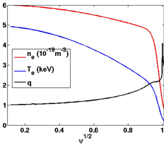
FIG. 1: Initial radial profiles at t = 0 for JET-like simulations: electron temperature T_e in keV , density n_e in 10^{19}m^{-3} and safety factor q . These profiles are typical experimental JET profiles (previously used in simulations in [17]); the q -profile is almost flat in the pedestal due to the bootstrap current.
