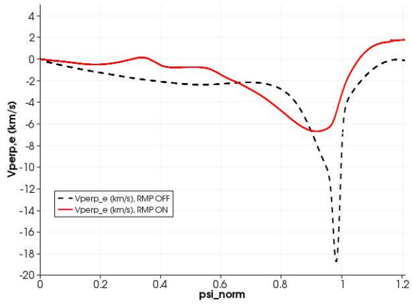
FIG. 60: Radial profile of the electron perpendicular velocity at the midplane in the LFS without RMPs (- - black) and with RMPs (red)
