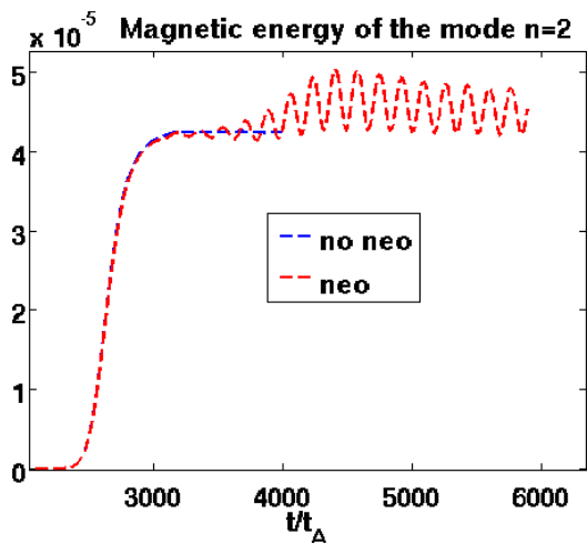
FIG. 21: Effect of the neoclassical friction on the magnetic energy of the driven mode n = 2 (resistivity \eta_0 = 10^{-7} ) at large diamagnetic rotation ( 2 \times 10^{-3} ). Without neoclassical effects in the model (in blue), the islands are static. With neoclassical friction included (in red), the generated islands are first static but finally rotate at the ion perpendicular rotation frequency.
