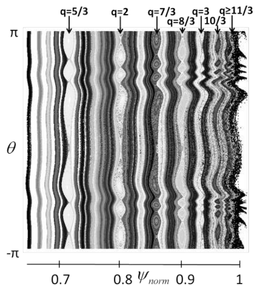
FIG. 36: Poincare plot of the magnetic topology with RMPs in (\psi, \theta) coordinates: magnetic field lines (starting at the edge inside the separatrix) integration after 200 toroidal turns at \varphi=0 . Resonant surfaces q=m/3 , m \geq 5 are indicated. A stochastic layer is formed for \psi \geq 0.96
