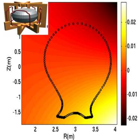
FIG. 3: cosine component of the n = 2 magnetic flux perturbation generated by EFCC for I_{coil} = 40kA . The black dots correspond to the boundary of the computational domain where the perturbations are applied.
