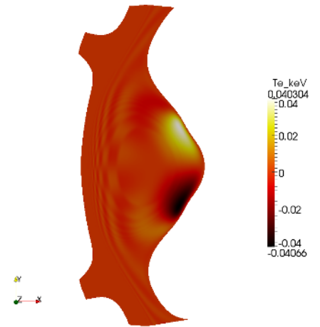
FIG. 50: Electron temperature perturbation with n = 3 RMPs in MAST (without diamagnetic effects)
