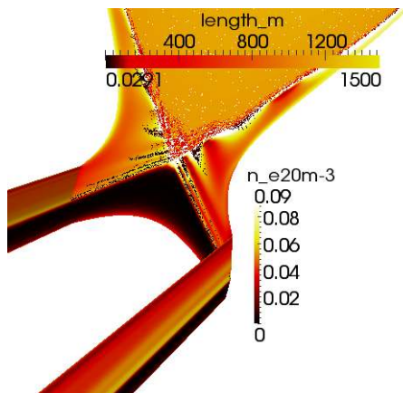
FIG. 43: Superposition of the 2D-plot (in the poloidal plane) of the magnetic topology (connection length) near the X-point with the electron density on the divertor targets (in the toroidal direction). Note the induced splitting of the strike points on the outer divertor target.
