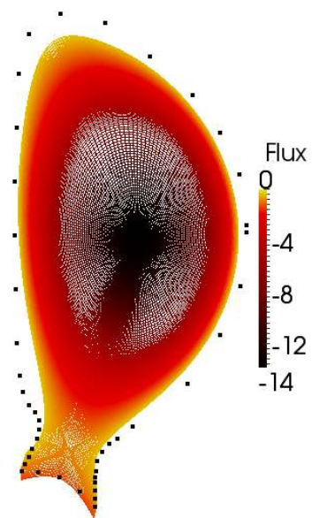
FIG. 24: ITER equilibrium flux-aligned mesh used in modeling
