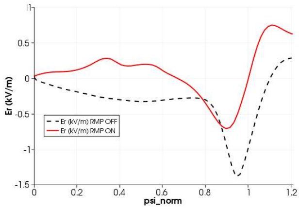
FIG. 59: Radial profile of the radial electric field at the midplane in the LFS without RMPs (- - black) and with RMPs (red)
