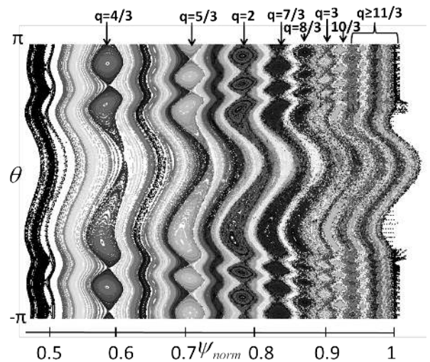
FIG. 53: Poincaré plot of the magnetic topology in MAST without diamagnetic rotation, in (\psi, \theta) coordinates: magnetic field lines integration after 200 toroidal turns. The resonant surfaces q = m/3 , m \geq 4 are indicated. A stochastic layer is formed for \psi \geq 0.96
