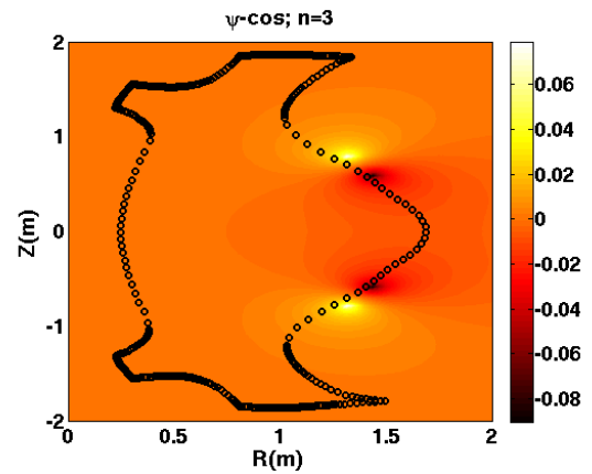
FIG. 45: Input resonant magnetic perturbation generated by the RMP coils calculated in the vacuum with the ERGOS code and applied as boundary conditions of the computational domain (in black)
