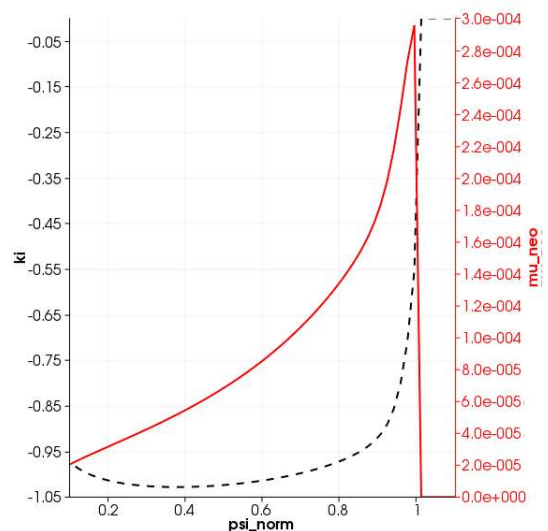
FIG. 2: Realistic radial profiles of the neoclassical coefficients k_i (left axis) and \mu_{i,neo} (right axis) used for simulations in the JET case.
