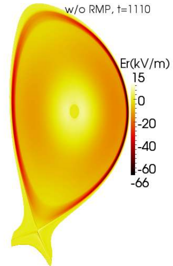
FIG. 27: 2D-profile of the radial equilibrium electric field in ITER (without RMPs)
