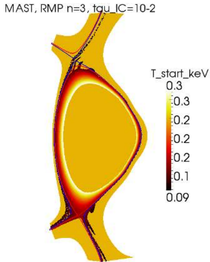
FIG. 55: Poincaré plot of the magnetic topology with diamagnetic flow. The color represents the temperature of the starting point of the field line inside the separatrices. The length of the lobes near the X-points is sensibly the same in the case without diamagnetic flow
