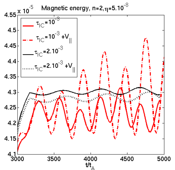
FIG. 20: Effect of the source of parallel rotation on the magnetic energy of the driven mode n = 2 (resistivity \eta_0 = 5 \times 10^{-8} ) at low ( \tau_{IC} = 10^{-3} ) and high ( 2 \times 10^{-3} ) diamagnetic rotation
