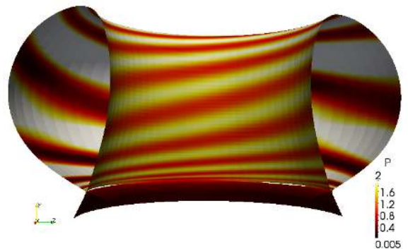
FIG. 40: 3D-plot of the pressure on an initial equilibrium flux surface without RMP near the separatrix. The 3D-deformation corresponds to a mode (n = 3, m \sim 12) .
