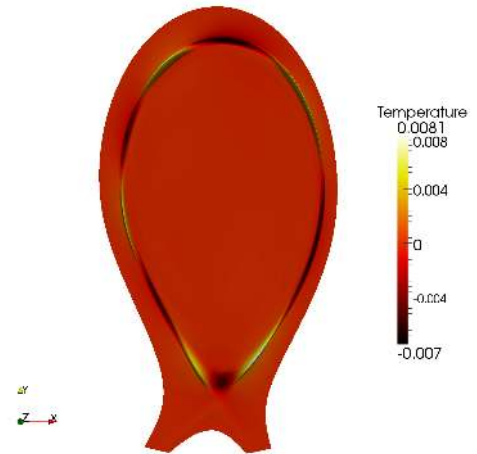
FIG. 16: n = 2 temperature perturbation with RMPs, mainly located on the resonant surface q = 5/2 ( \eta_0 = 10^{-7} , \tau_{IC} = 10^{-3} )
