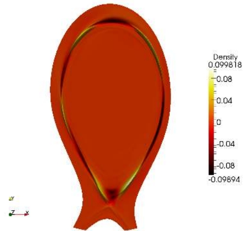
FIG. 15: n = 2 density perturbation with RMPs, mainly located on the resonant surface q = 5/2 ( \eta_0 = 10^{-7} , \tau_{IC} = 10^{-3} )
