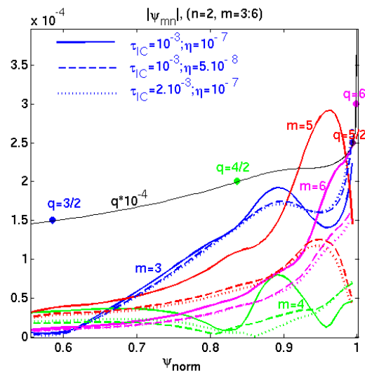
FIG. 19: Fourier harmonics of the magnetic flux ( n = 2 , m = 3 - 6 ) depending on the resistivity and the diamagnetic rotation
