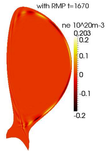
FIG. 31: n = 3 density perturbation due to RMPs in ITER
