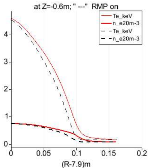
FIG. 33: Density and temperature profiles at the edge for Z=-0.6\text{m} without (full line) and with RMPs (dash)
