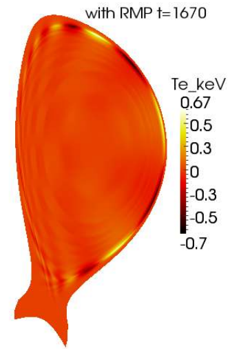
FIG. 32: n = 3 temperature perturbation due to RMPs in ITER
