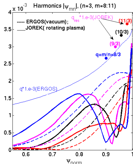
FIG. 35: Fourier harmonics of the magnetic flux perturbation |\psi_{m,n}| , n=3 , m=8-11 in the vacuum case (ERGOS code, dash) and taking into account the plasma response (JOREK, full line). The q -profile is given and the positions of the resonant surfaces are indicated by the dots. The edge harmonics m=10-11 have a comparable amplitude on the resonant surfaces q=10-11/3 in the ERGOS and JOREK cases, showing the penetration of these harmonics in the plasma.
