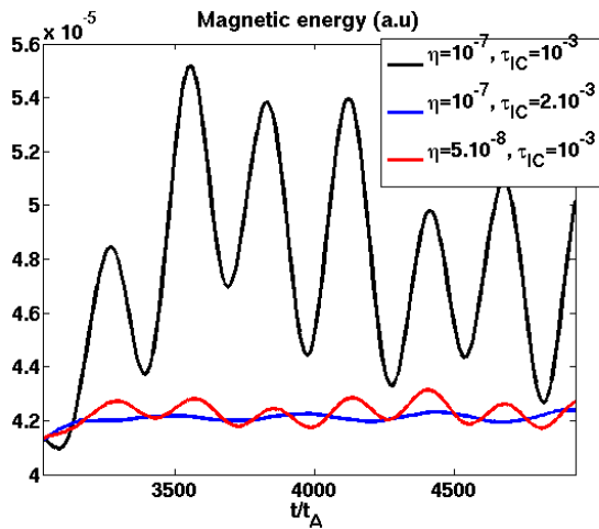
FIG. 17: Three different regimes of penetration of the RMPs: magnetic energy of the mode n = 2 depending on the diamagnetic parameter \tau_{IC} and the plasma resistivity \eta_0
