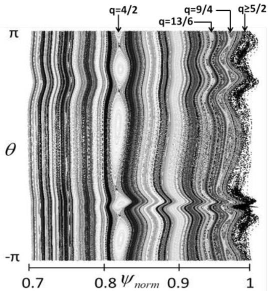
FIG. 13: Poincaré plot of the magnetic topology in (\psi, \theta) coordinates ( \eta_0 = 10^{-7} , \tau_{IC} = 10^{-3} )
