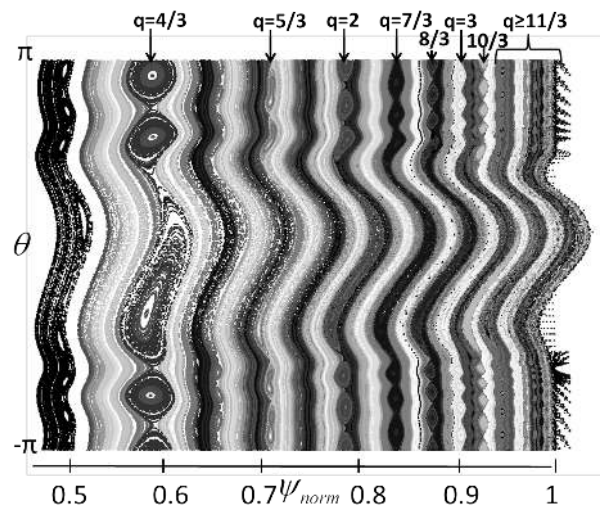
FIG. 54: Poincaré plot of the magnetic topology in MAST with diamagnetic rotation included, in (\psi, \theta) coordinates: magnetic field lines integration after 200 toroidal turns. The resonant surfaces q = m/3 , m \geq 4 are indicated. A stochastic layer is formed for \psi \geq 0.96
