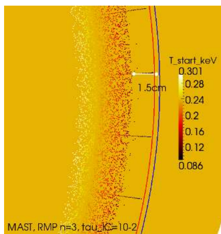
FIG. 56: Zoom in Poincaré plot Fig. 55 around the midplane (case with diamagnetic flow): the displacement of the last closed flux surface due to RMPs at the toroidal angle \varphi = 0^\circ is approximately 1.5cm
