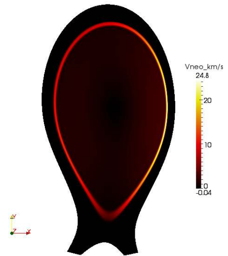
FIG. 6: Neoclassical velocity (in km/s) in JET
