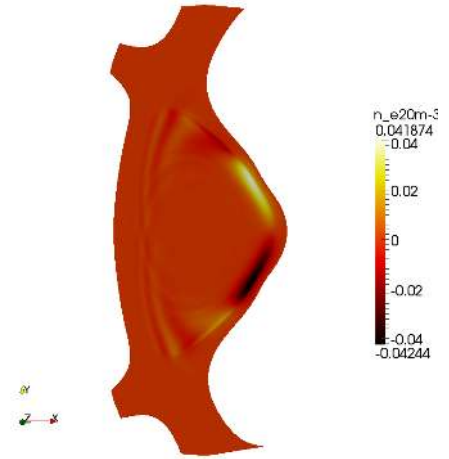
FIG. 49: Density perturbation with n = 3 RMPs in MAST (without diamagnetic effects)
