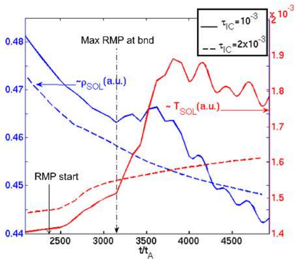
FIG. 18: Volume integrated electron density and temperature in the Scrape-off layer at resistivity \eta_0 = 10^{-7} for two different diamagnetic velocities ( \tau_{IC} = 10^{-3} and 2 \times 10^{-3} ).
