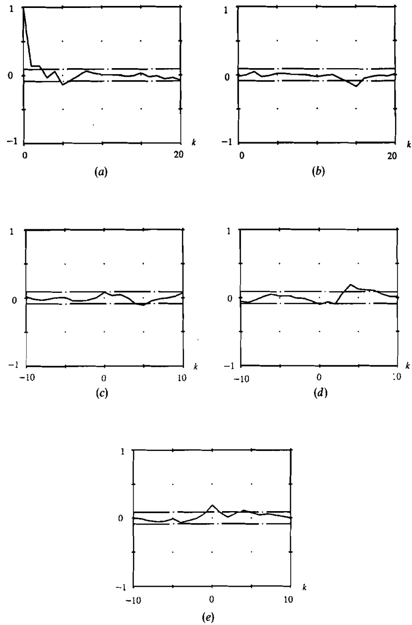
Figure 11. Correlation tests using test set (Example 3): (a) \Phi_{ee}(k) ; (b) \Phi_{e(ea)}(k) ; (c) \Phi_{ue}(k) ; (d) \Phi_{u^2e}(k) ; (e) \Phi_{u^2e^2}(k) . Dashed line: 95% confidence interval.
