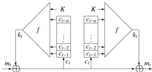
Figure 1: Self Synchronizing Stream Cipher model
