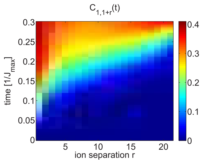
Extended Data Figure 2 | Numeric calculation of XY model correlations. Calculated spatial and time-dependent correlations for an N = 22 -spin XY model with spin-spin couplings J_{ij} \approx J_0/|i-j|^{1.19} , found by numerically evolving the Schrödinger equation.
