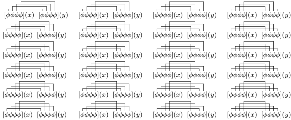
Figure 1. The 4! different Wick contractions leading to the topology of last diagram in (2.8).
