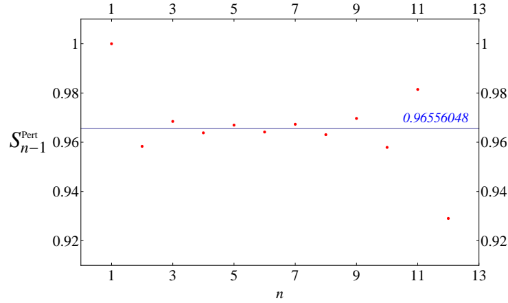
Figure 2. S_{n-1}^{\text{Pert}} ( n \in \{1, \dots, 12\} ), for \lambda = \frac{1}{3} , compared to the exact result (2.11) (horizontal line).
