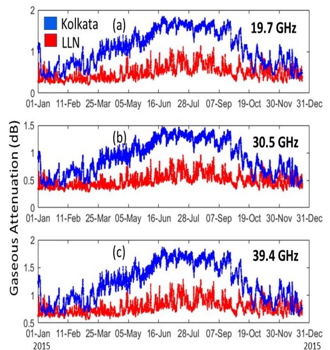
FIGURE 10. Gaseous attenuation over Kolkata and LLN during the time period January 2015 to December 2015 for: (a) 19.7 GHz, (b) 30.5 GHz and (c) 39.4 GHz.
