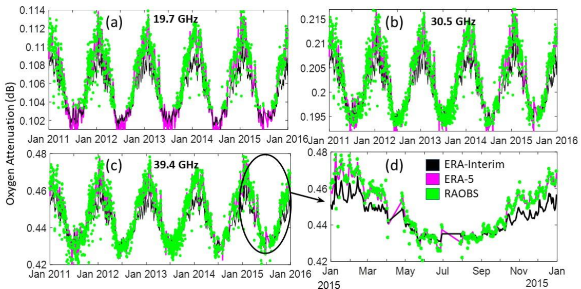
FIGURE 1. Time series of oxygen attenuation over Kolkata at 29.8^\circ elevation angle at frequencies: (a) 19.7 GHz, (b) 30.5 GHz and (c) 39.4 GHz, and (d) Variation of oxygen attenuation over Kolkata during January 2015 to December 2015 at Q band (39.4 GHz).
