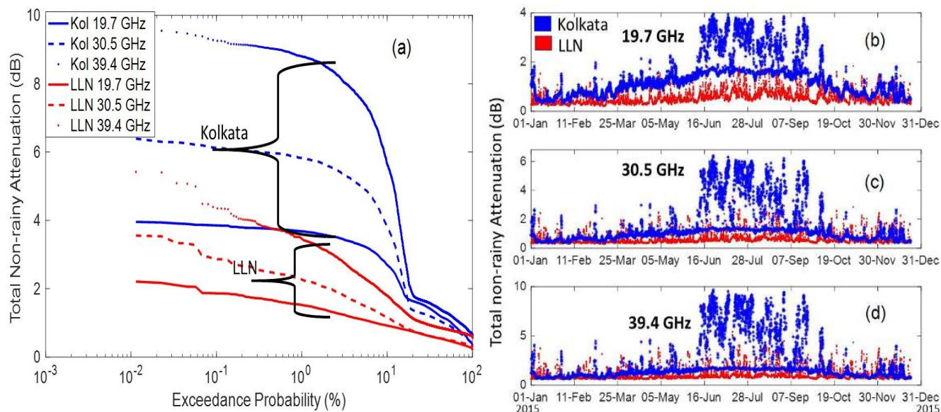
FIGURE 11. (a) Exceedance probability of total non-rainy attenuation from ERA-5 data sources over Kolkata and LLN during 2015 and, Total non-rainy attenuation (dB) over LLN and Kolkata during the time period January 2015 to December 2015 for: (b) 19.7 GHz, (c) 30.5 GHz, (d) 39.4 GHz.
