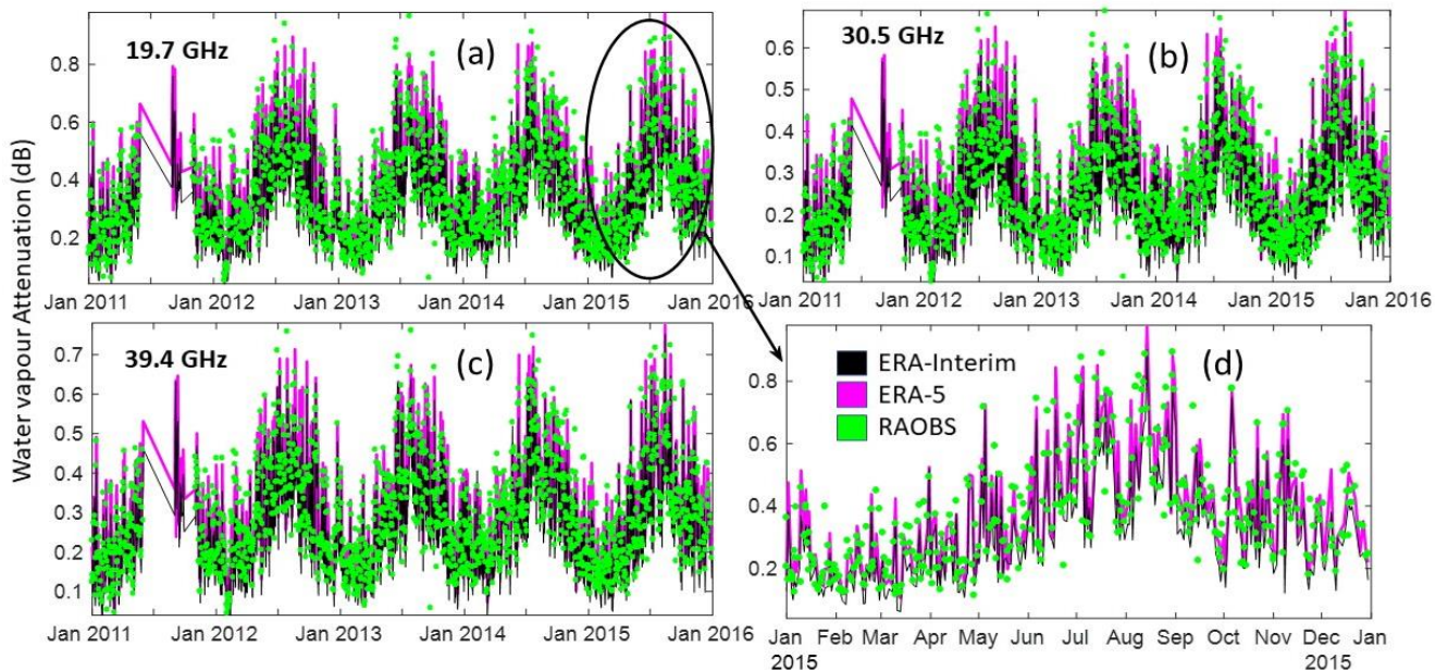
FIGURE 5. Time series of water vapour attenuation over LLN at 29.8^\circ elevation angle at frequencies: (a) 19.7 GHz, (b) 30.5 GHz and (c) 39.4 GHz, and (d) Variation of water vapour attenuation over LLN during January 2015 to December 2015 at K band (19.7 GHz).
