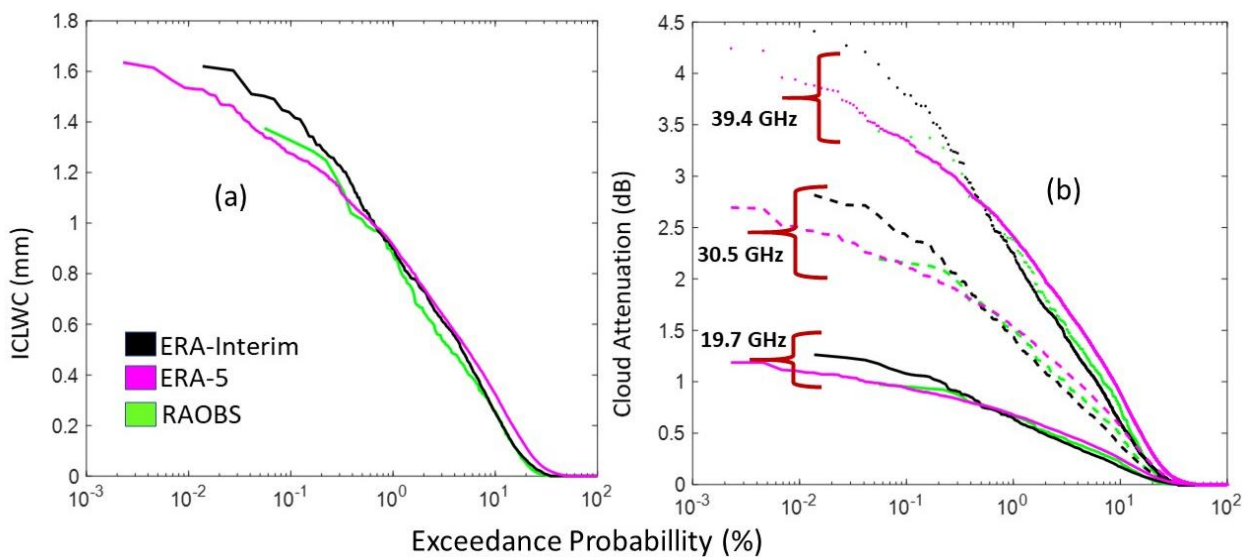
FIGURE 8. Exceedance probability of (a) ICLWC and (b) cloud attenuation, obtained from RAOBS, ERA-5 and ERA-Interim data over LLN at 29.8° during 2011-2015.
