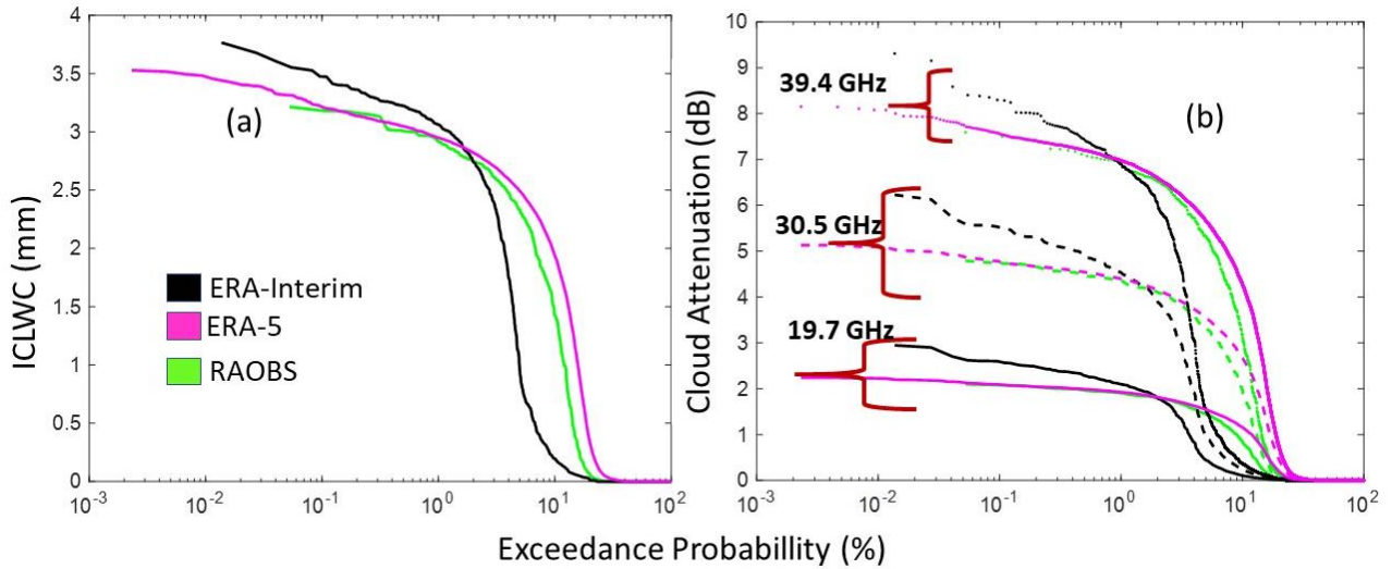
FIGURE 7. Exceedance probability of (a) ICLWC and (b) cloud attenuation, obtained from RAOBS, ERA-5 and ERA-Interim data over Kolkata at 29.8° during 2011-2015.
