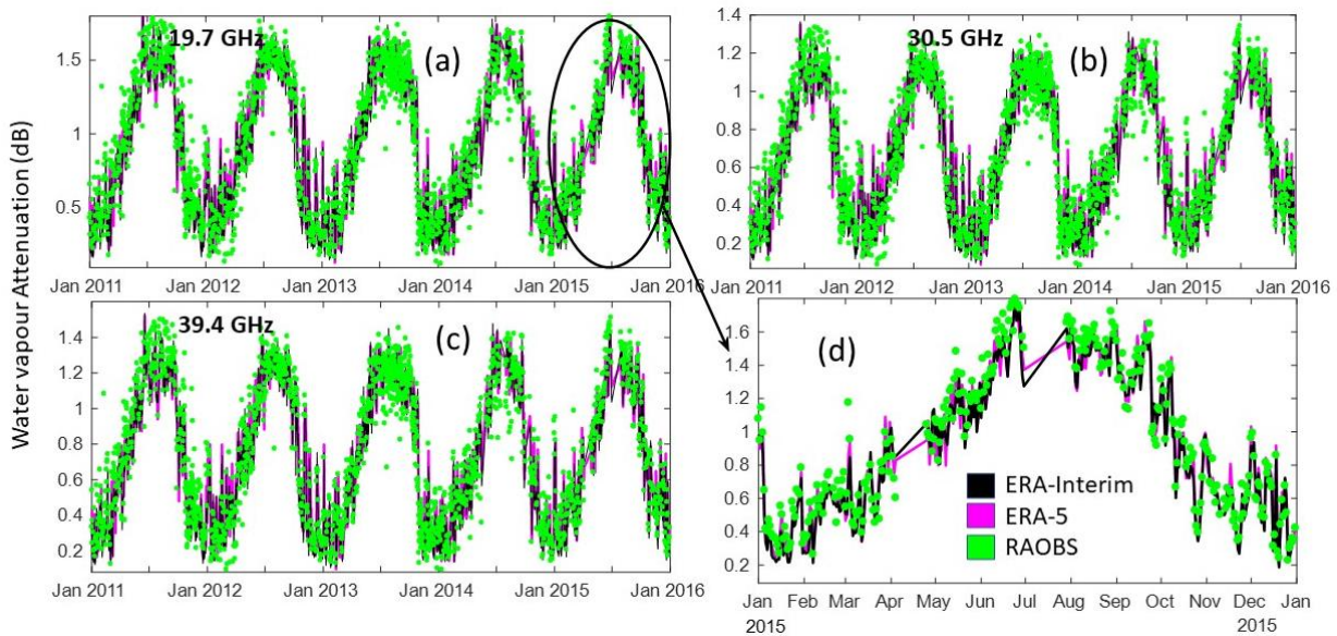
FIGURE 4. Time series of water vapour attenuation over Kolkata at 29.8^\circ elevation angle at frequencies: (a) 19.7 GHz, (b) 30.5 GHz and (c) 39.4 GHz, and (d) Variation of water vapour attenuation over Kolkata during January 2015 to December 2015 at K band (19.7 GHz).
