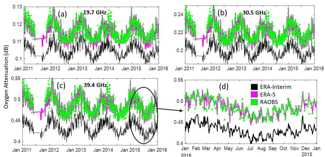
FIGURE 2. Time series of oxygen attenuation over LLN at 29.8^\circ elevation angle at frequencies: (a) 19.7 GHz, (b) 30.5 GHz and (c) 39.4 GHz, and (d) Variation of oxygen attenuation over LLN during January 2015 to December 2015 at Q band (39.4 GHz).
