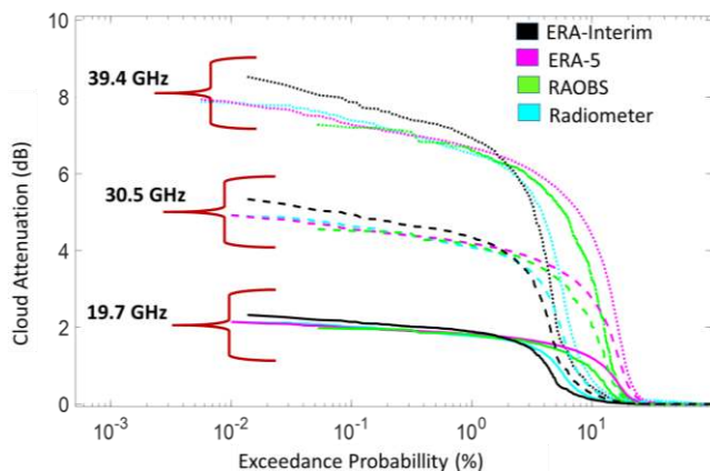
FIGURE 9. Exceedance probability of cloud attenuation from various meteorological data sources over Kolkata at 29.8°.
