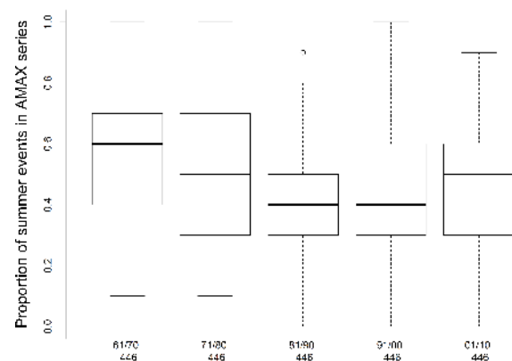
Fig. 4. Proportion of summer events in the annual maximum rainfall series, shown separately for each decade. The number of catchments used to compute the proportions is indicated below the x axis.
