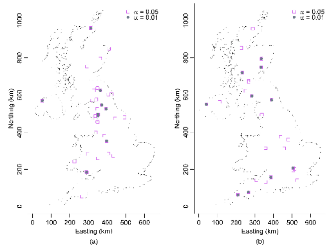
Fig. 12. (a) Sites for which the null hypothesis H_0 : \beta_1 \leq \log(1.2)/85 is rejected. (b) Sites for which the null hypothesis H_0 : \beta_1 > \log(1.2)/85 is rejected. Results shown for two different significance levels \alpha = 0.05 and \alpha = 0.01 .
