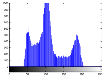
Figure 15. x) Histogram plot of original image in 24.a)
