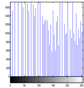
Fig 4: Histogram of output image after global histogram equalization
