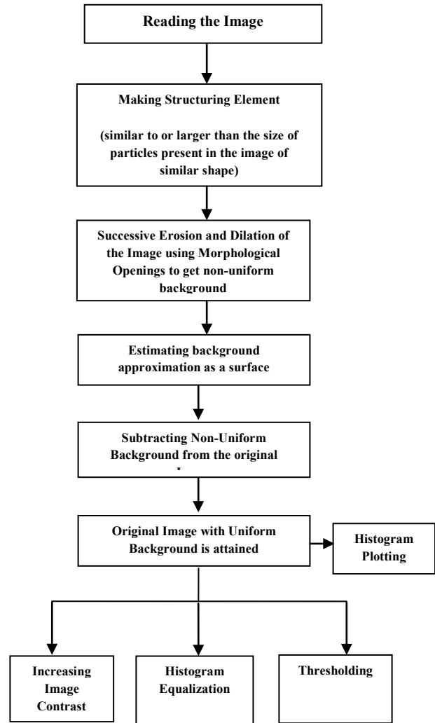
Fig.11: Algorithm Designed for non-uniform background removal for particle analysis and image enhancement
