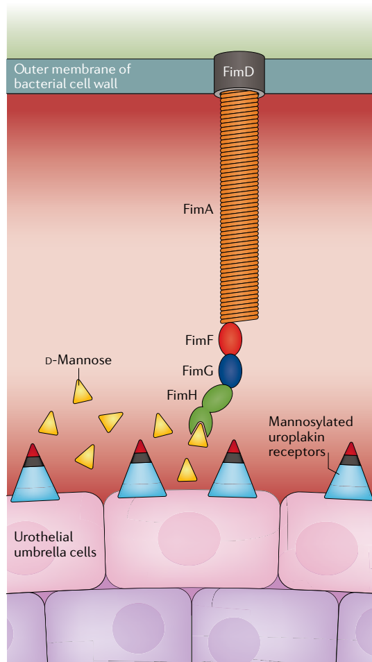
Fig. 7 | D-Mannose prevents binding of bacteria to urothelial cells. D-Mannose is similar in structure to the binding site of urothelial glycoprotein receptors (such as uroplakin) and, therefore, can cause saturation of FimH adhesins and prevent bacteria from binding to urothelial glycoprotein receptors if present in sufficient concentration in the urine.
