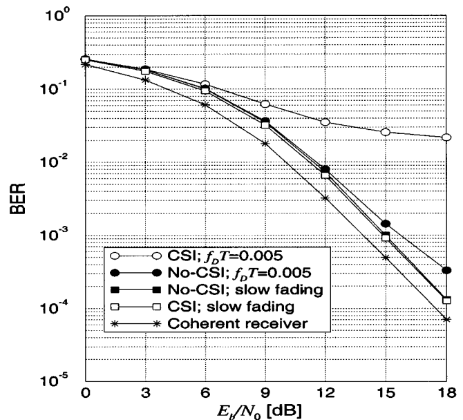
Fig. 2. BER of the proposed receivers with and without CSI, S = 4 and N = 3 , for differentially encoded 16-QAM and Rice fading with K_R = 10 dB. The performance of an ideal coherent receiver is also shown for comparison.
