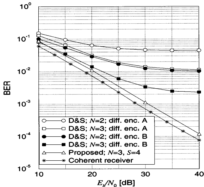
Fig. 4. BER of the proposed receiver without CSI, S = 4 and N = 3 , for differentially encoded 16-QAM and slow Rayleigh fading, and comparison to that of the receivers in [14] (D&S).
