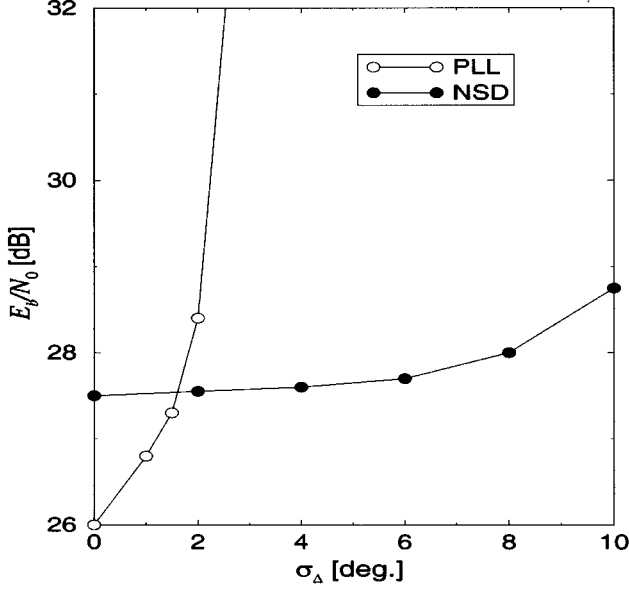
Fig. 6. E_b/N_0 as a function of the phase noise standard deviation for BER equal to 10^{-3} of the proposed receiver without CSI, S = 1 and N = 4 , for differentially encoded QPSK, slow Rayleigh fading (black marks), and comparison to a coherent receiver based on a decision-directed PLL (white marks).
