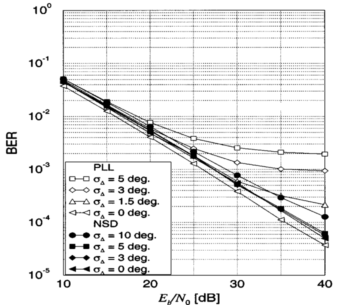
Fig. 5. BER of the proposed receiver without CSI, S = 1 and N = 4 , for differentially encoded QPSK, slow Rayleigh fading, various values of phase noise standard deviation (black marks) and comparison with a coherent receiver based on a decision-directed PLL (white marks).
