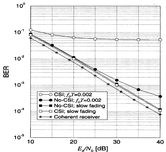
Fig. 3. BER of the proposed receivers with and without CSI, S = 4 and N = 3 , for differentially encoded 16-QAM and Rayleigh fading. The performance of an ideal coherent receiver is also shown for comparison.
