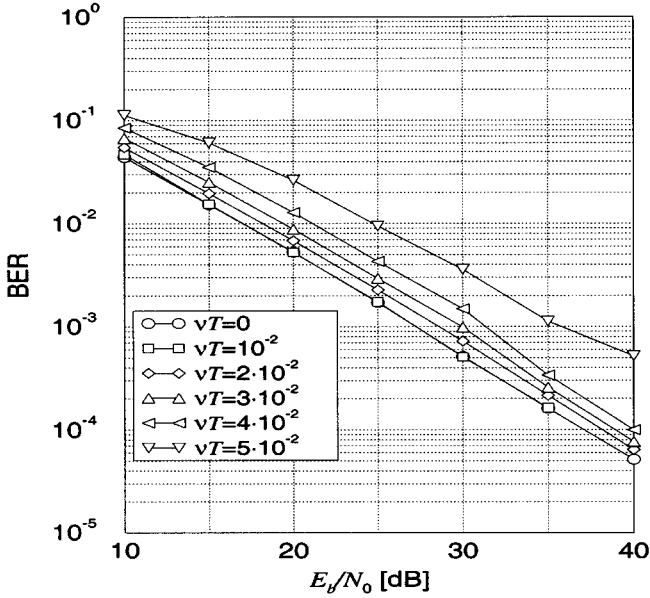
Fig. 7. BER of the proposed receiver without CSI, S = 1 and N = 4 , for differentially encoded QPSK, slow Rayleigh fading, and various values of the normalized frequency offset.
