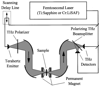
FIG. 1. Schematic of the experimental setup used for the measurements of the THz Hall effect. The apparatus is similar to that of Ref. 12, with the addition of a 1.3 T permanent magnet with optical access, a free-standing wire grid polarizing beamsplitter, and a second THz detector, oriented at 90^\circ to the first. The THz emitter is oriented at 45^\circ , to emit diagonally polarized radiation.
