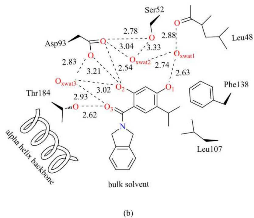
Figure 10. BIIB02 and VHD interactions with environment, according to crystal structure with PDB: 3O6O, 2XAB
