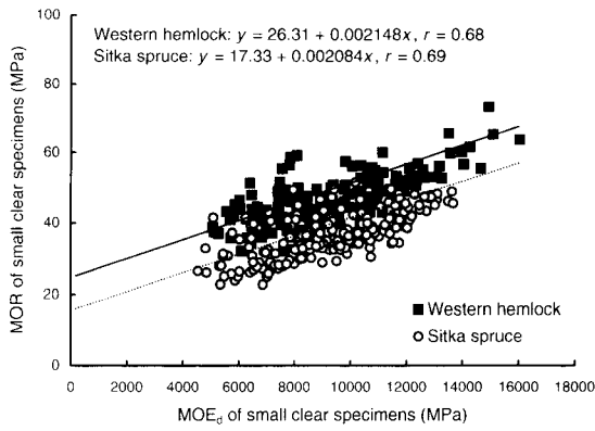
FIG. 6. Relationship of MOE_d to MOR for small, clear specimens.
