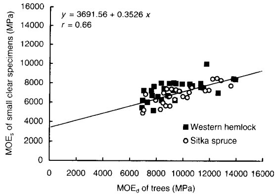
FIG. 8. Relationship of MOE_d of trees to MOE_s of small, clear specimens.
