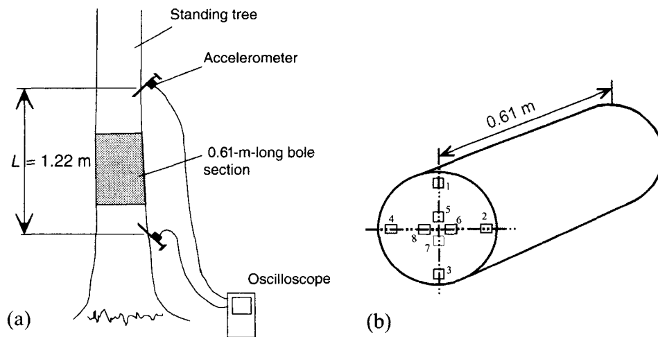
FIG. 2. (a) Experimental setup used in field test, and (b) cutting pattern for small, clear wood specimens.
