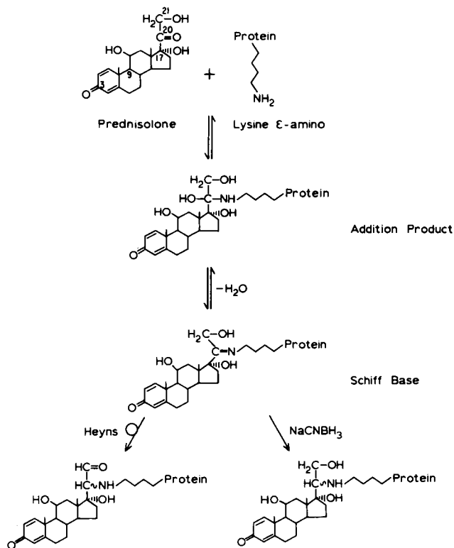
Figure 1. The reaction scheme between the glucocorticoid, prednisolone, and the lysine residues of proteins, showing the adducts formed by the proposed Heyns rearrangement and by the addition of \text{NaCNBH}_3 .
