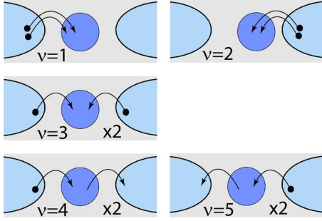
FIG. 4. (Color online) Elementary processes for the transitions |0\rangle \rightarrow |2\rangle and |0\rangle \rightarrow |0\rangle . The label “ \times 2 ” signals an additional factor of 2 due to two incoherent spin contributions. The diagrams for the processes corresponding to the transitions |2\rangle \rightarrow |0\rangle and |2\rangle \rightarrow |2\rangle are obtained by reversing the direction of all arrows.
