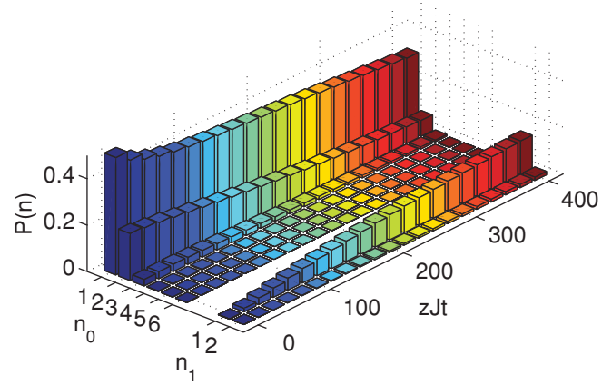
FIG. 10. (Color online) Particle number statistics for the lowest band and one of the three first excited bands, computed for an interacting system with U/(zJ) = 1 as a function of time using a Gutzwiller ansatz for the system density operator. As in Fig. 9, we choose \gamma^{(0,0,0,0)} = 0.01zJ in an isotropic 3D lattice ( z = 6 ) of depth V = 10E_R .
