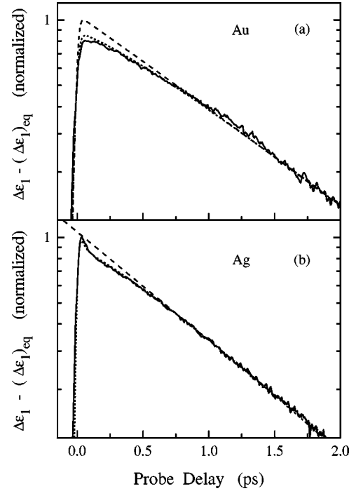
FIG. 9. (a) Measured transient change of \Delta\varepsilon_1 in a 25-nm Au film at \hbar\omega_{pr} = 1.45 eV on a logarithmic scale (full line). The dotted and dashed lines are the interband contribution to \Delta\varepsilon_1 computed for the transient electron distribution and for a thermal electron gas, respectively. (b) Measured \Delta\varepsilon_1 in a 23-nm Ag film for \hbar\omega_{pr} = 2.9 eV (full line). The dashed line shows an exponential decay with \tau_{e-ph} = 850 fs. The dotted line is the average of the calculated \Delta\varepsilon_1 using the Rosei and parabolic models.
