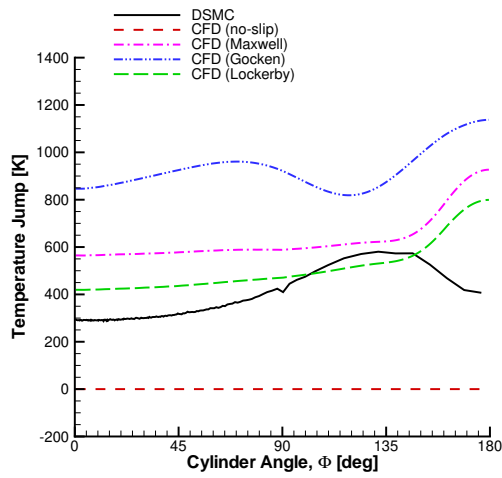
(c) Kn = 0.05
