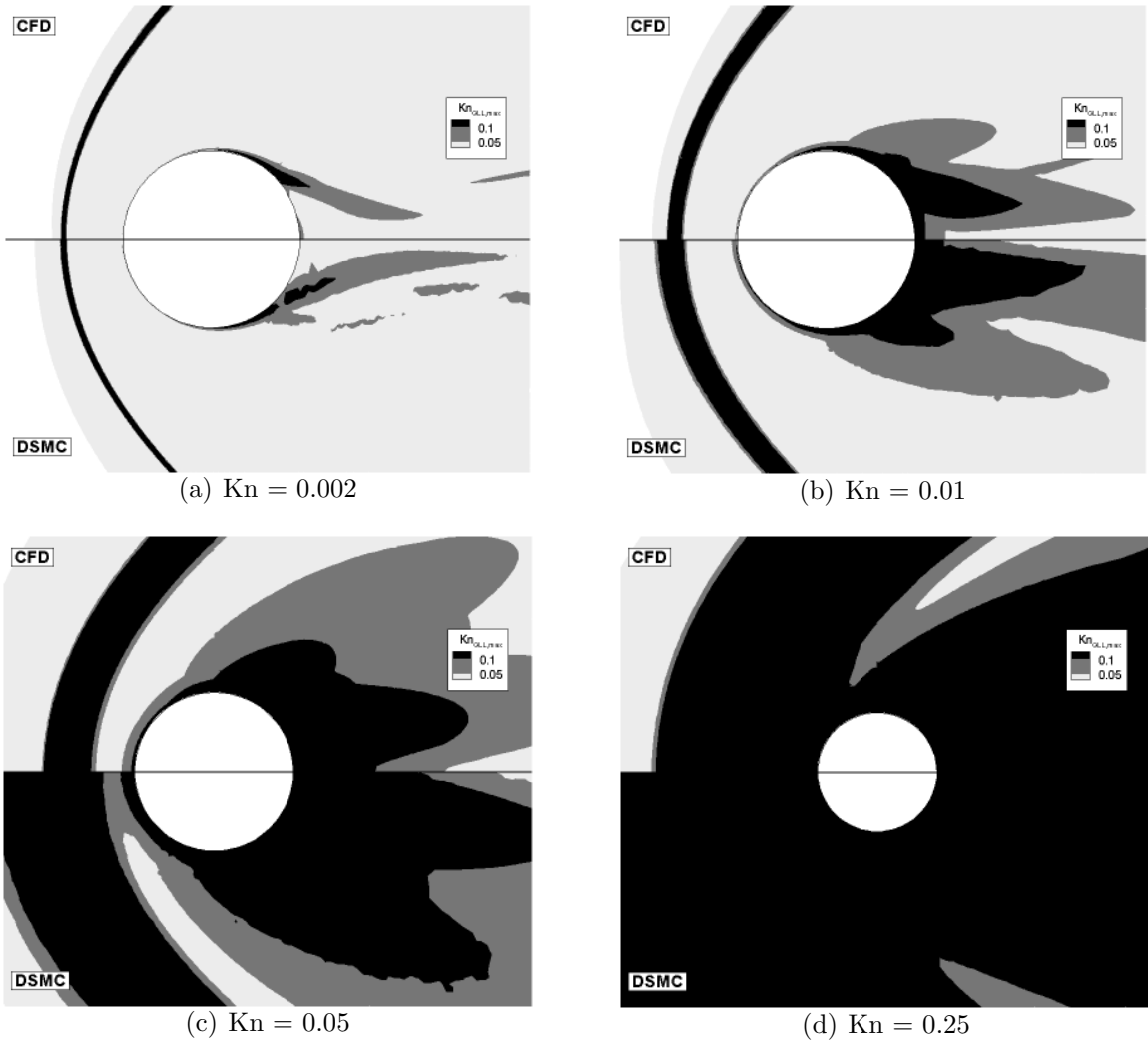
Figure 4.6: Kn_{GLL} field for a Mach 10 flow of argon about a cylinder. Light gray regions correspond to Kn_{GLL} < 0.05 , dark gray regions correspond to 0.05 < Kn_{GLL} < 0.1 and black regions correspond to Kn_{GLL} > 0.1
