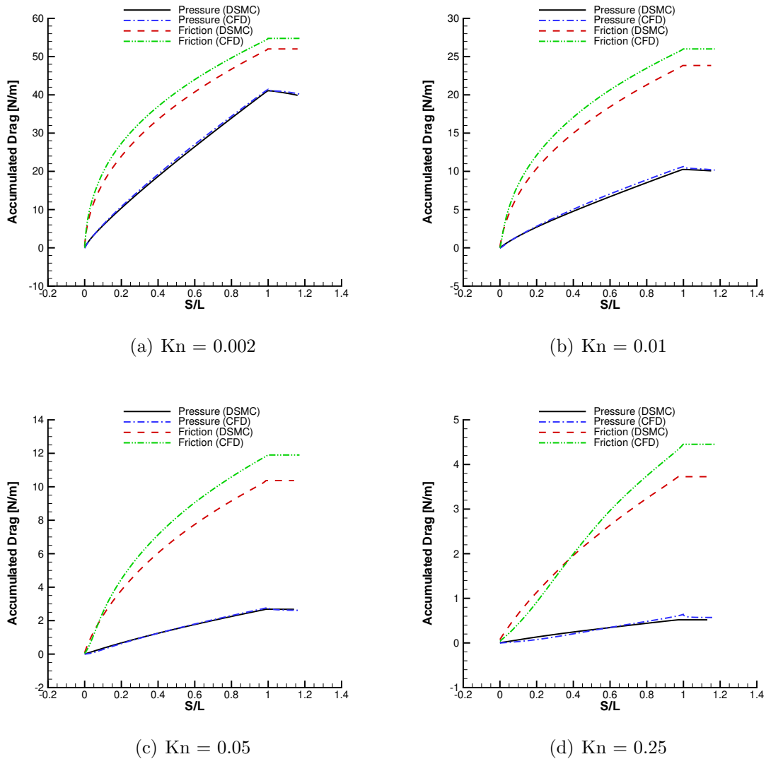
Figure 5.39: Contributions of pressure and skin friction forces to accumulated total drag for a Mach 25 flow of nitrogen about a wedge. The distance along the surface (including the base), S , is normalized by the top surface length, L .
