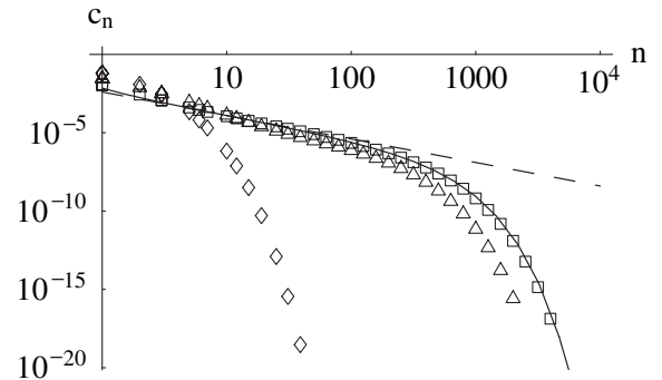
FIG. 2. The steady-state domain size distribution for MDRR recycling with \phi = j_{on}/j_{off} = 0.1 , j_{off} \tau_D = 10^{-3} , and \gamma = 2 ( \diamond ), 4 ( \triangle ), and 6 ( \square ). The mean domain contains 1.3, 2.3, and 5.3 monomers, respectively, rather small because a fast recycling rate was chosen for numerical convenience. The asymptotic variation for large line tensions Eq. (7) is shown (solid line) as is Eq. (8) (dashed line) appropriate for sizes 1 \ll n \ll \bar{n}^2 .
