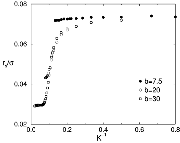
FIG. 4. Localization length (root-mean-square displacement) r_s in the glass along the critical glass transition lines in Fig. 2 as a function of the reduced temperature K^{-1} for various values of the Yukawa screening parameter b , as labeled.
