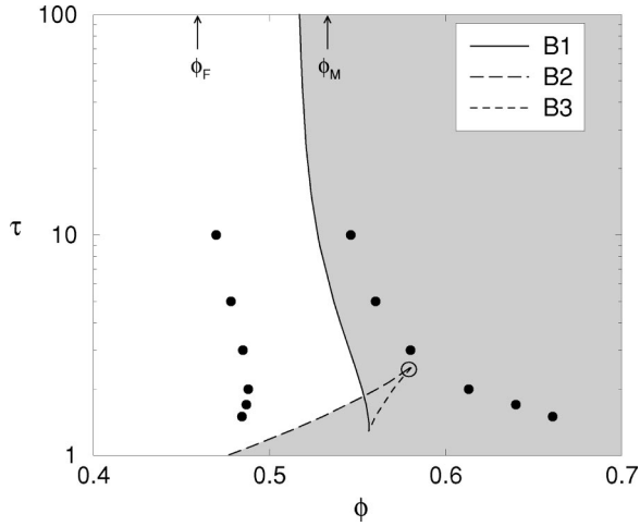
FIG. 1. AHS phase diagram in terms of the reduced temperature \tau and the particle volume fraction \phi . The labeled lines are the bifurcation lines of Eq. (1) discussed in the text. The shaded region encloses nonergodic density fluctuations. Liquid-glass transitions occur when crossing the B1 and B2 lines into the shaded nonergodic region. Glass-glass transitions occur along the piece of the B2 line inside the nonergodic region. The physically relevant endpoint singularity is indicated by a circle. The data for the fluid-solid freezing and melting lines ( \bullet ) are taken from MWDA calculations [55]. The arrows show the (PY) hard sphere freezing ( \phi_F ) and melting ( \phi_M ) volume fractions [55].
