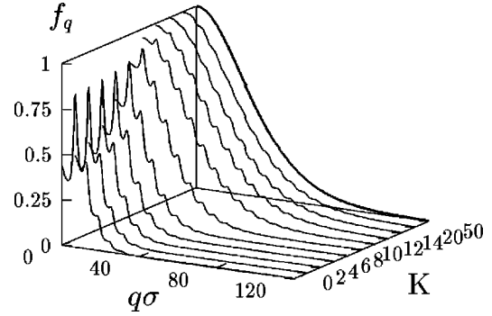
FIG. 3. HCA critical coherent nonergodicity parameters f_q for b=30 as functions of normalized wave vector q\sigma and Yukawa prefactor K . Note that the volume fraction varies according to the b=30 critical glass transition line in Fig. 2, and that the K values jump from K=14-20 and 50 . The rear curve shown in bold is the density and temperature independent asymptotic prediction resulting from Eq. (8) and b \rightarrow \infty .
