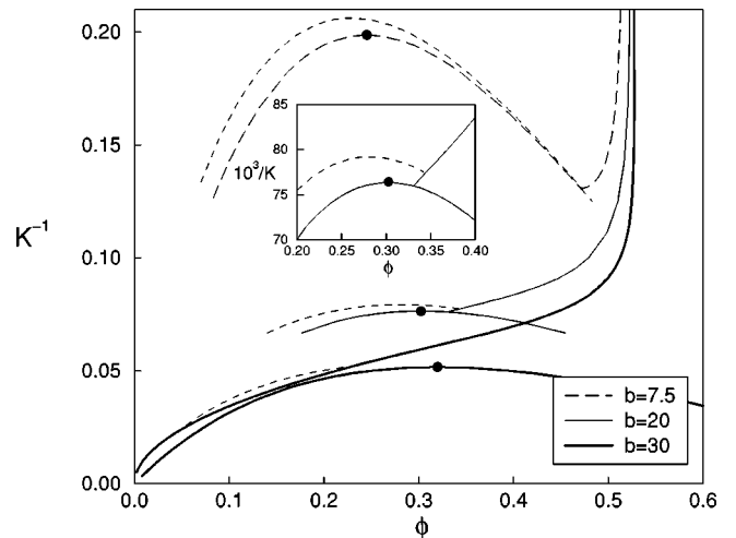
FIG. 7. HCAY phase diagrams showing, in addition to the MSA gas-liquid spinodal curves and the MCT glass transition lines as in Fig. 2, the MCT transition lines (short-dashed lines) which are characterized by a small- q structural arrest in f_q and f_q^s = 0 . The inset shows an enlargement of the line crossing in the vicinity of the b = 20 critical point.
