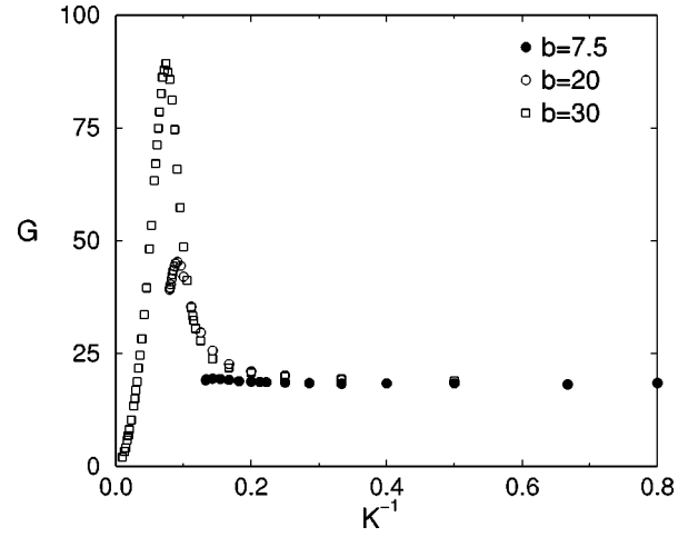
FIG. 5. Elastic shear modulus (in units of kT/\sigma^3 ) in the glass along the critical glass transition lines in Fig. 2 as a function of the reduced temperature K^{-1} for various values of the Yukawa screening parameter b , as labeled.
