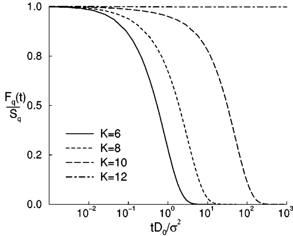
FIG. 6. Normalized intermediate scattering function at a fixed wave vector q\sigma=0.2 as a function of Yukawa prefactor and dimensionless time, as labeled. The corresponding locations in the b=20 HCAY diagram are shown in Fig. 2 as open circles.
