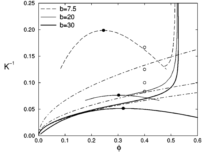
FIG. 2. HCAY phase diagrams in terms of the reduced temperature K^{-1} and particle volume fraction \phi for varying values of the screening parameter b , as labeled. MSA gas-liquid spinodals are shown with critical points denoted by (●), together with the corresponding MCT glass transition lines as labeled. The chain curves correspond to the asymptotic prediction in Eq. (8) with \Gamma_c(b \rightarrow \infty) = 3.02 . The open circles (○) denote the locations in the b=20 diagram of the suspensions for which the results in Fig. 6 were calculated.
