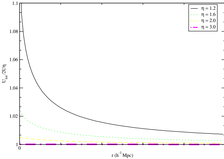
Fig. 2. Correlation energy ratio for \eta models. For comparison, the Hernquist’s model is computed for \eta = 2 .
