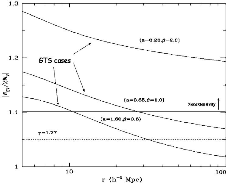
Fig. 1. Behaviour of the correlation energy ratio with the scale R .
