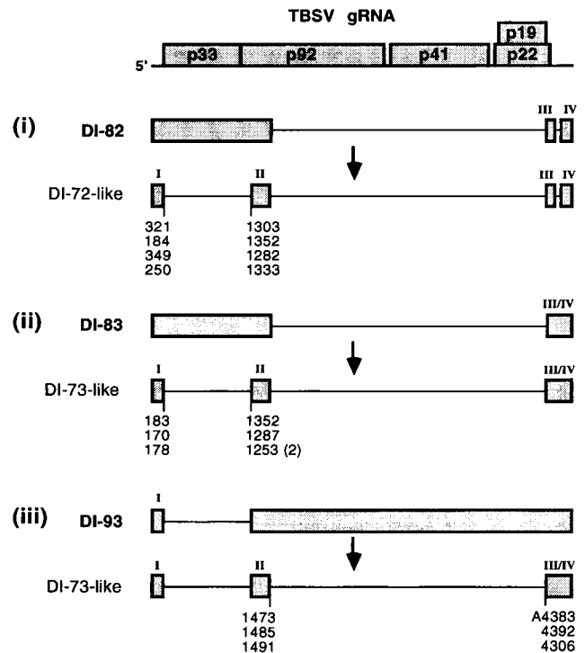
FIG. 9. Schematic representation of the transitions of large putative DI RNA precursors to smaller DI RNA species after a single passage. The gRNA of TBSV is shown schematically at the top, and the transitions observed for DI-82, DI-83, and DI-93 are shown below. The coordinates given correspond to those of the gRNA of TBSV (10). The number in parentheses in diagram ii indicates that two independent clones contained that junction. The letter A in front of the coordinate in diagram iii represents an inserted adenosine residue at that junction.
