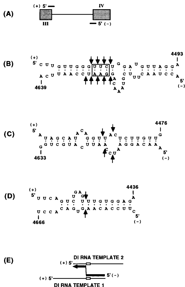
FIG. 11. Stepwise deletion model for generation and evolution of tombusvirus DI RNAs. Panels: A, viral gRNA; B, large DI RNA precursors; C, DI-73-like molecules; D, DI-72-like molecules; E, DI RNA containing a duplicated segment. See the Discussion for details.
