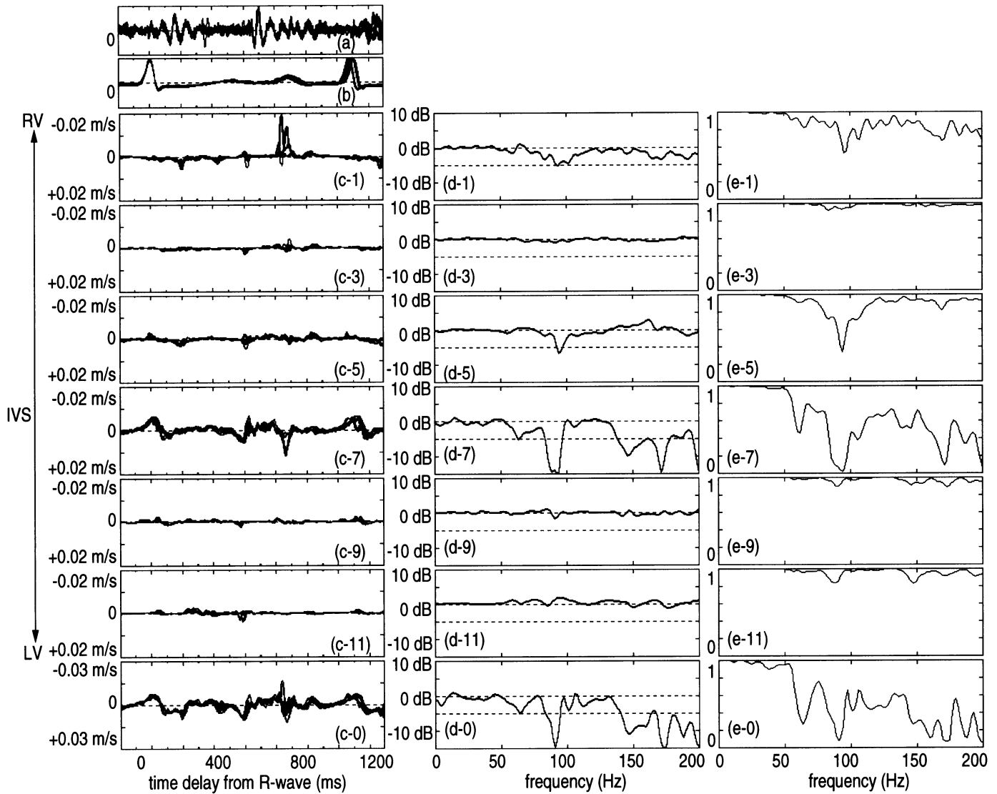
Fig. 10. The instantaneous speed \Delta_t h_i(t) of the thickness change of (10), the transfer function H(x_i \rightarrow x_{i+2}; f) from v(x_i; t) to v(x_{i+2}; t) , and the coherence function, estimated in 6 regions in the IVS for the 8 heartbeats of the serious patient in Figs. 6(3) and 9. The measurement was performed two months before his death. (For details see Fig. 8.)
