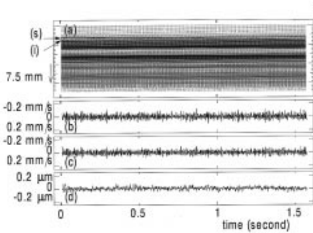
Fig. 3. Experimental results for evaluation of measurable lower limit using a water tank. (a): The object motion x_s(t) and x_i(t) estimated by the proposed method, superimposed on the M-mode image obtained by the magnitude of the received signal. (b) and (c): The velocity signal estimates v(x_s; t) and v(x_i; t) of points (s) and (i). (d): The change in thickness, h(t) , between point (i) and (s) obtained from v(x_s; t) and v(x_i; t) .
