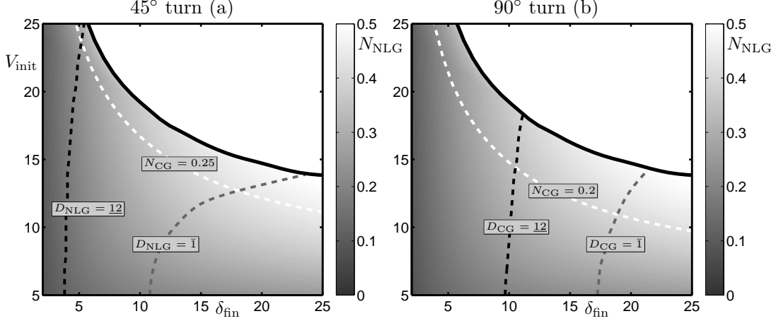
Figure 7: Greyscale maps show the lateral NLG load N_{NLG} for the trajectory represented by each (\delta_{fnn}, V_{init}) -pair. The operating regions are represented by the values of \delta_{fnn} and V_{init} that lie inside bounds on D_{NLG} , D_{CG} and N_{CG} as shown.
