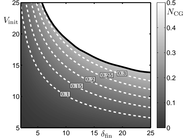
Figure 6: Greyscale map of the maximal lateral load factor N_{CG} for the output trajectory initialised from each (\delta_{\text{fin}}, V_{\text{init}}) -pair; dashed white curves are contours of N_{CG} .
