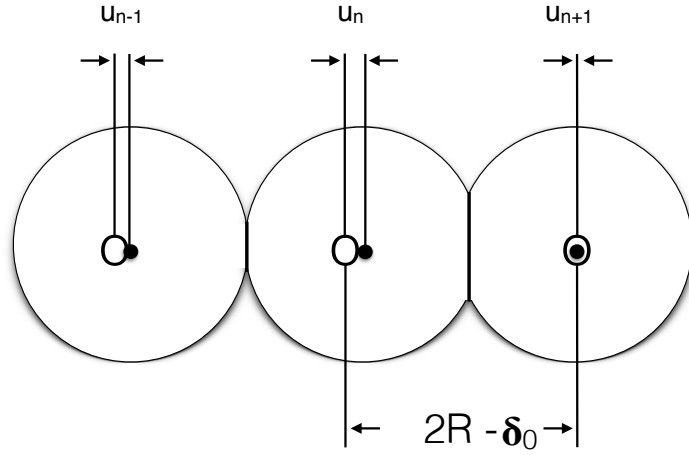
Figure 2: One-dimensional monomer granular chain compressed by a static force F_0 . The open circles represent the initial positions of the particle centers in static equilibrium, and the black circles indicated the displaced positions. [This figure was inspired by Ref. [136].]
