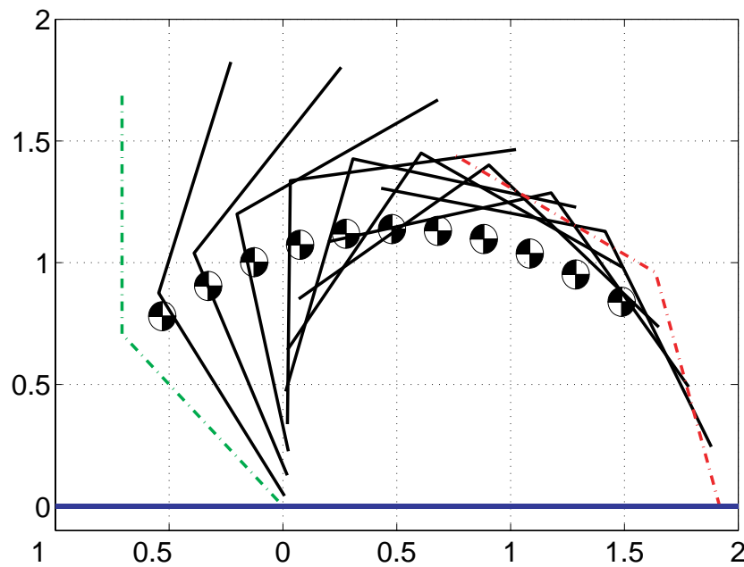
Fig. 9. The motion of the robot passes from left to right without passing through a singularity. The initial configuration ( \cdot - \cdot - green) and final configuration ( \cdot - \cdot - red) belong to the same configuration class. The center of gravity follows a parabolic trajectory.
