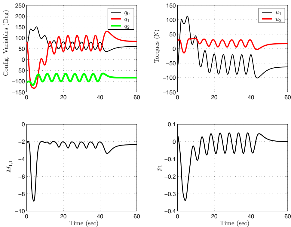
Fig. 7. Demonstration of asymptotic tracking and stabilization for the three-link mechanism; see Figure 6 for details. The plots show the configuration variables (upper left), joint torques (upper right), coefficient that determines invertibility of the decoupling matrix (lower left), and the function that is the key to designing the proper set of outputs (lower right).
