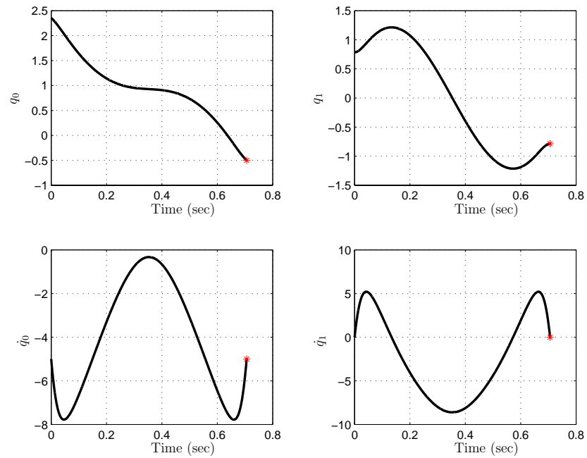
Fig. 14. The computed open-loop control transfers the robot from its initial state to the desired final state (*).
