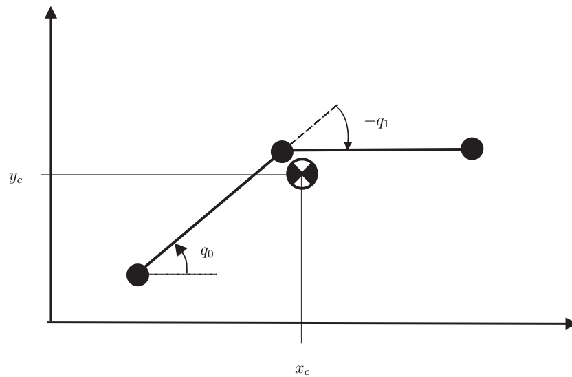
Fig. 8. A two-link robot undergoing ballistic motion in a vertical plane. Only the joint q_1 is actuated. From left to right, the links have length L_1 and L_2 and the masses are m_0, m_1, m_2 .
