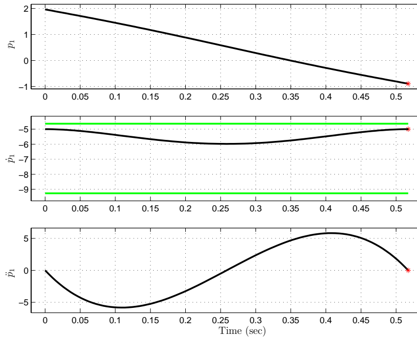
Fig. 10. Based on the initial and final conditions of the flight phase, a trajectory for p_1 and its derivatives is derived. The plot shows that \dot{p} satisfies the constraint \frac{\sigma}{a_{00}-a_{01}} \leq \dot{p}_1(t) \leq \frac{\sigma}{a_{00}+a_{01}}
