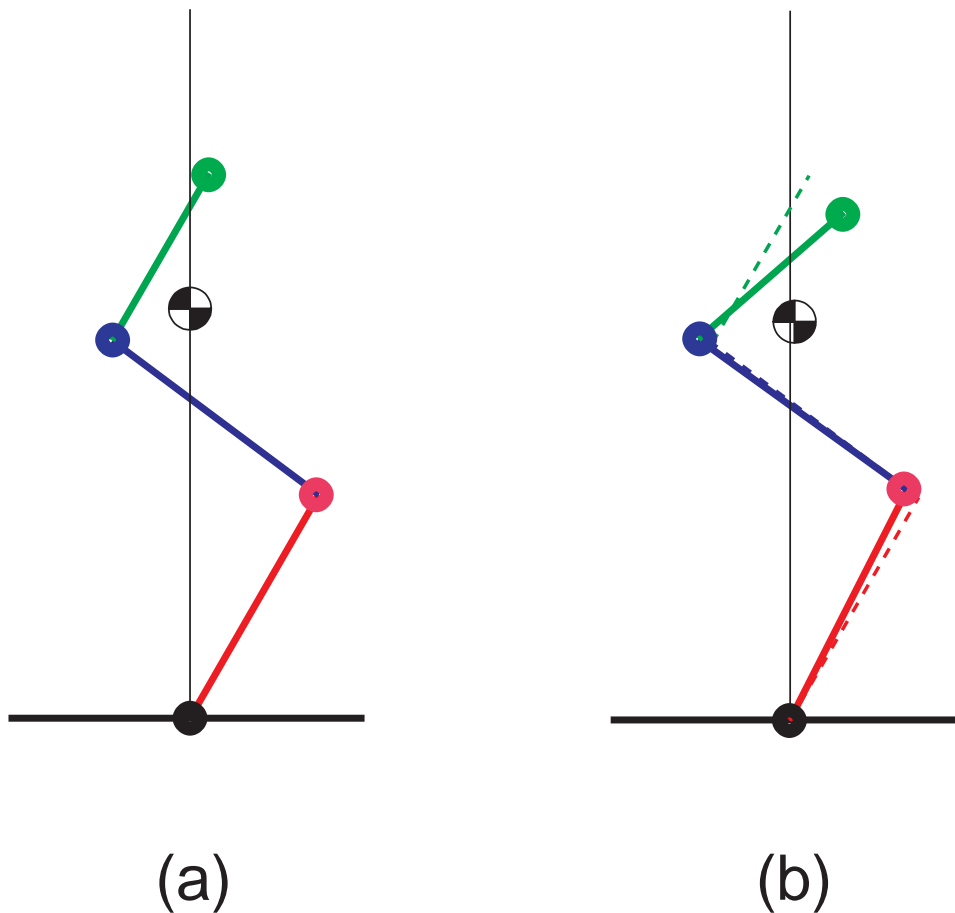
Fig. 5. Three-link mechanism, connected at a pivot, consisting of point masses and massless bars. The links have length L_1 through L_3 starting at the pivot; the masses are m_1 through m_3 . (a) shows an equilibrium pose with the center of gravity centered over the pivot; (b) shows the initial condition used in the simulation, with the equilibrium position superimposed in the background.
