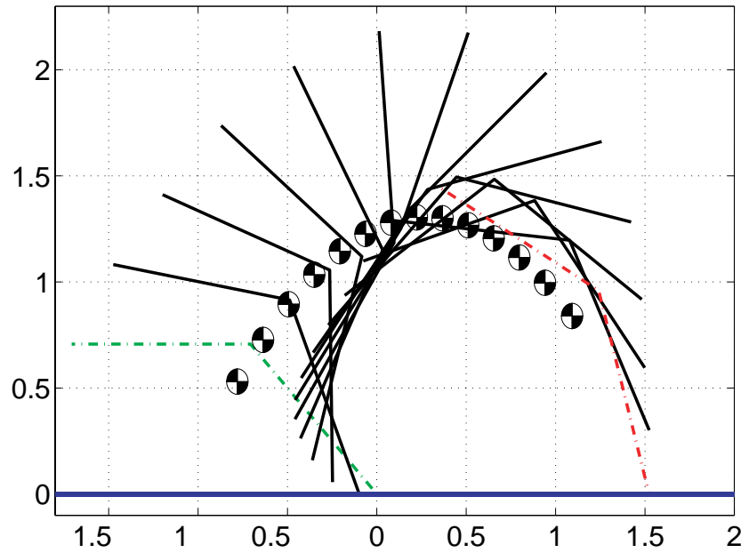
Fig. 12. The motion of the robot passes from left to right, with a singular position occurring when the two links are aligned. The initial configuration (· - · green) and final configuration (· - · red) belong to different configuration classes.
