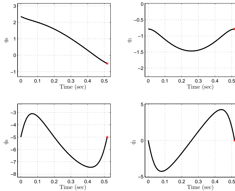
Fig. 11. The computed open-loop control transfers the robot from its initial state to the desired final state (*).
