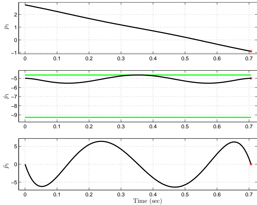
Fig. 13. Based on the initial and final conditions of the flight phase, a trajectory for p_1 and its derivatives is derived. The plot shows that \dot{p}_1 hits the constraint \frac{\sigma}{a_{00}+a_{01}} in the middle of the flight phase, which allows the change in the configuration class to occur.
