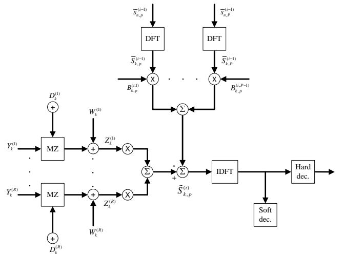
Fig. 5. Multiuser IB-DFE receiver design.
