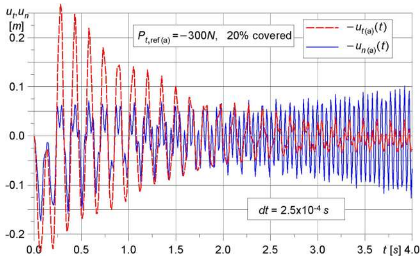
Fig. 28 Controlled response, 2-patch, 20% covered ( t = 4 s)
