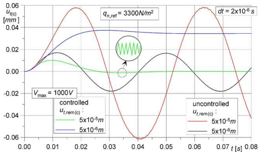
Fig. 57 Middle point tangential displacements versus time for a step load q = 3300\text{N/m}^2
