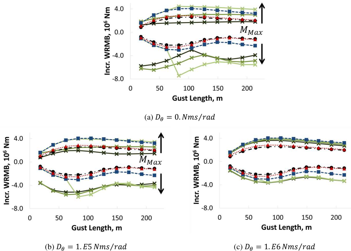
Figure 12. WRBM Envelopes for Different Hinge Moments Threshold and Hinge Damping Values (Lg=83m)
