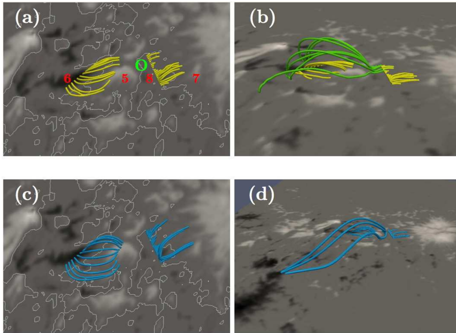
Figure 9. (a) The emerging sea-serpent above the \text{PIL}_\Omega s of Figure 8 imaged with yellow field lines, in orthogonal projection. The vertical field B_z is shown in grey-scale in the background, together with the PIL (in white). The green circle indicates the portion of the \text{PIL}_U where bald patches are found, and from where the green field lines of the right panel are started. (b) Perspective from a southern point of view of the magnetic configuration above the PILs. Green field lines are computed from points lying 0.5'' above the bald patch at the \text{PIL}_U (cf. Figure 8), while the yellow lines are the same than in the left panel. (c) As for panel (a) but for the potential field. (d) As panel (b) but for the potential field and a larger field of view.
