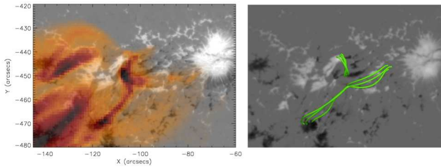
Figure 12. Left: XRT image obtained with the Ti poly filter on 4 July 2009 at 11:52 UT, aligned on the SOT/SP LOS image of 4 July 2009 at 11:58 UT, in reversed colour scale. Right: Same reconnected field lines as the green field lines in Figure 10c,d, projected on the plane of the sky.
