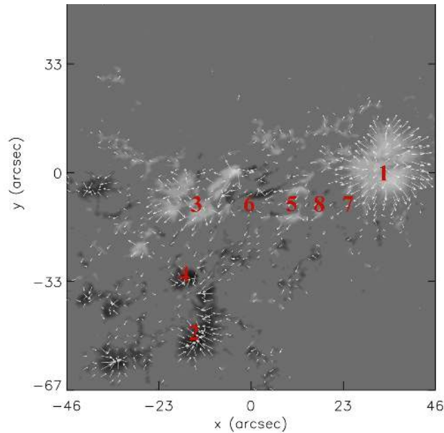
Figure 1. Vector magnetogram used as the boundary condition for the extrapolation, in the heliographic plane. The vertical field, ranging from -2409 G to 2965 G, is given in grey-scale and the transverse component is indicated by arrows, with the longest arrow corresponding to 2018 G. Only values of the transverse field above 100 G are depicted. The main polarities involved in the analysis are numbered (even and odd numbers are used for positive and negative polarities, respectively). The polarity pairs are associated both by the photospheric field evolution and by the magnetic field extrapolation in Section 6, and they have consecutive numbers). The photospheric field is derived from the SOT/SP scan on 4 July 2009 from 11:58 UT until 12:34 UT. The heliographic plane is tangent to the Sun at the central pixel of SOT/SP FOV, located at (-107'', -488'') in heliocentric coordinates, where the cartesian reference system employed in the extrapolation is centered. In these coordinates, the uniform spatial resolution of the extrapolated vector magnetogram is 0.32'' in both directions.
