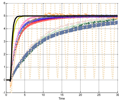
Fig. 3: Trajectory Gradient descent optimization in FMCTC
