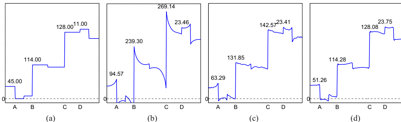
Fig. 5. (a) A scan line of a test image of vertical edges. (b)-(d) Contrast enhancement results of the test image with different methods: (b) global high pass filtering (“unsharp masking”), (c) local gamma correction in wavelet domain, (d) global gamma correction in DNT domain. Parameters in each operation were chosen so that the smallest intensity jump in the test image (point D) would be boosted to the same value.
