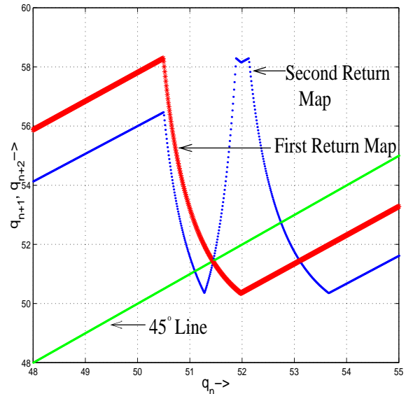
Fig. 4. 1. Red curve shows first return map, 2. blue curve shows second return map, and 3. green line is 45^\circ line whose intersection denotes the fixed points of the map
