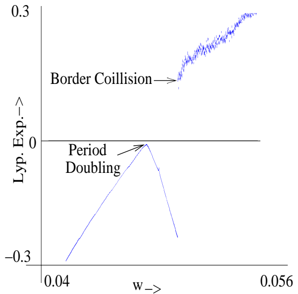
Fig. 8. Lyapunov exponent computed for average queue length w.r.t. w , p_{max} = 0.1
