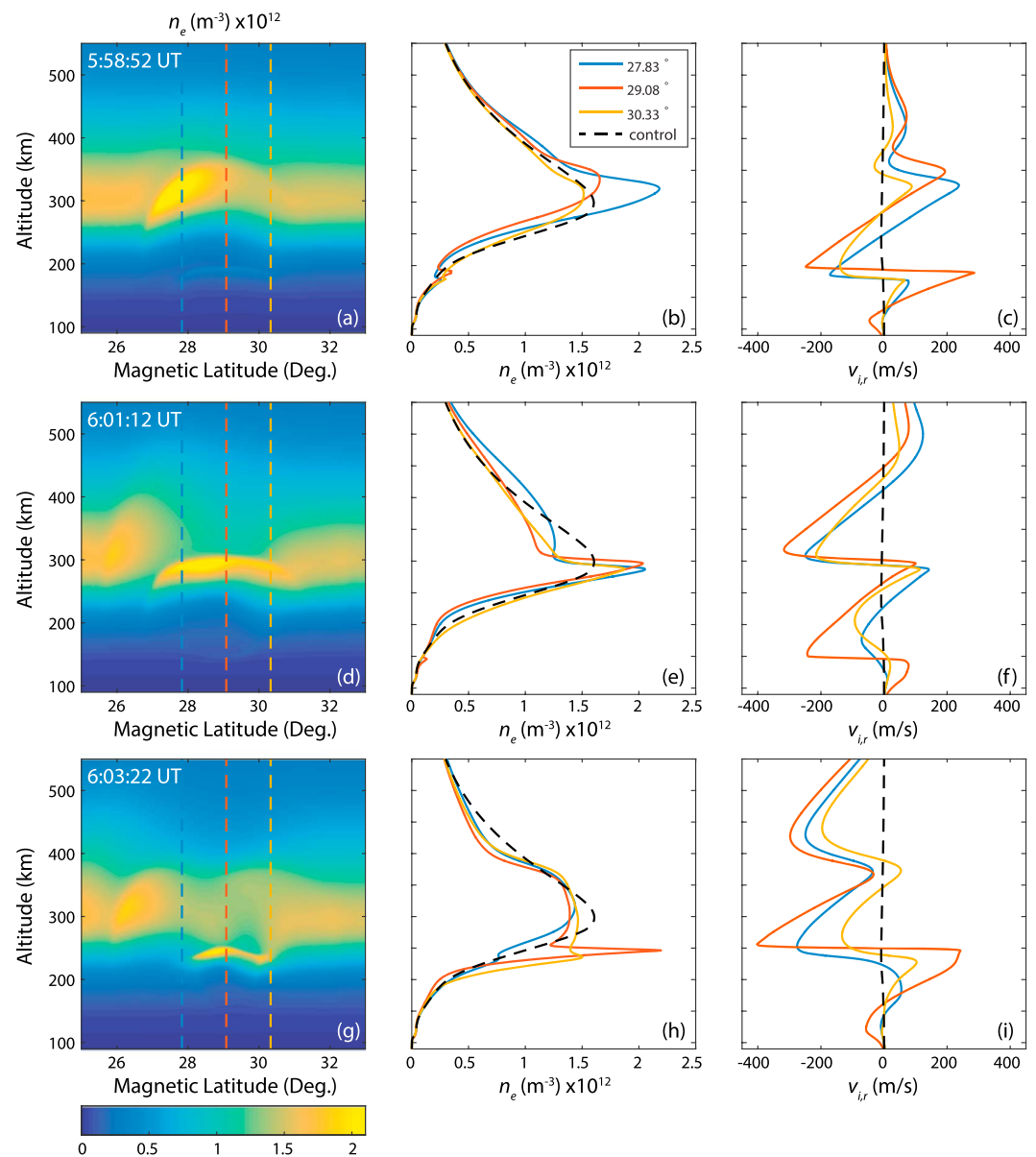
Figure 3. Simulated ionospheric density and velocity responses at different times over the epicenter for the 2011 Tohoku case study. Each row of figures represents a snapshot in time (as marked in the first panel of each row). (a, d, and g) Electron density versus altitude and magnetic latitude. (b, e, and h) Electron density profiles extracted from the three locations with corresponding line colors in Figures 3a, 3d, and 3g. The dashed black line shows what the electron density over the epicenter would be in absence of a perturbation (a control simulation). (c, f, and i) Vertical ion velocity extracted from three locations corresponding to the dashed lines in Figures 3a, 3d, and 3g (the control simulation velocity is, likewise, shown as a black dashed line in these plots).
