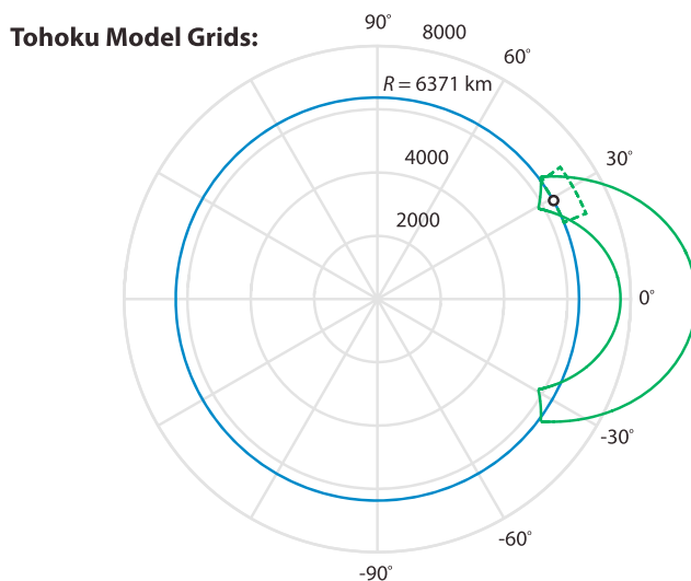
Figure 1. Atmospheric-ionospheric dynamics model grids used in this study. The green dashed lines mark the edges of the atmospheric dynamics module, while the green solid lines give outline of the ionospheric module. The surface of the Earth is marked by a blue line. The acoustic wave sources used in this study are located at sea level in the “horizontal” center of the atmospheric dynamics mesh (indicated by the open circle in the figure).
