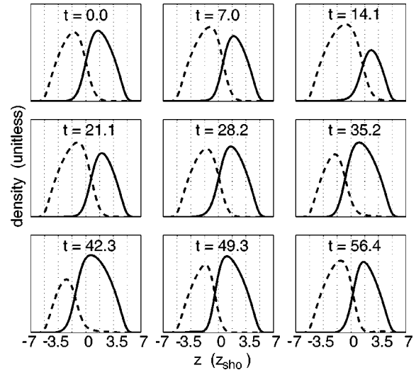
FIG. 2. Plot showing the time-evolution of the density of each component. The x axis is the position z , and the time t of each snapshot is shown. This case corresponds to the solid line plotted in Fig. 1. The detuning is \delta = -0.39 , chosen so that the system is initially being driven on resonance.
