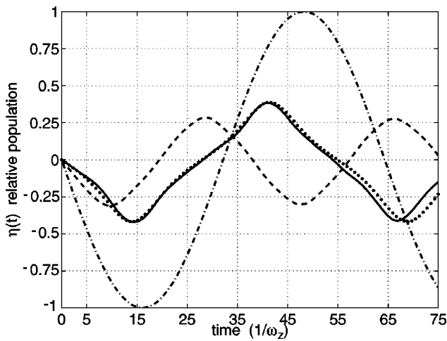
FIG. 1. Plot showing oscillations of the relative population. The dashed-dot line corresponds to the case where the mean-field interaction has been set to zero, the initial relative phase is \phi(0) = \pi/2 , and \delta = 0 . The dashed line is for the same initial relative phase of \pi/2 , but with the mean-field interaction turned on and \delta = -0.39 . The solid line is for \phi(0) = 3\pi/16 and \delta = -0.39 . The three lines described are solutions of Eq. (1), whereas the dotted line is a solution of Eq. (7) with the same parameters as for the solid line.
