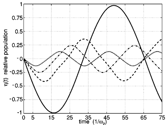
FIG. 3. Plot showing that the effect of the displacement z_0 on the system is to suppress the amplitude of oscillation. The four curves represent increasing values of z_0 : 0 (solid), 0.1 (dashed), 0.2 (dash-dotted), and 0.5 (dotted). In each case, the detuning \delta is chosen so that the system is initially being driven resonantly, and the initial phase is \phi(0) = \pi/2 .
