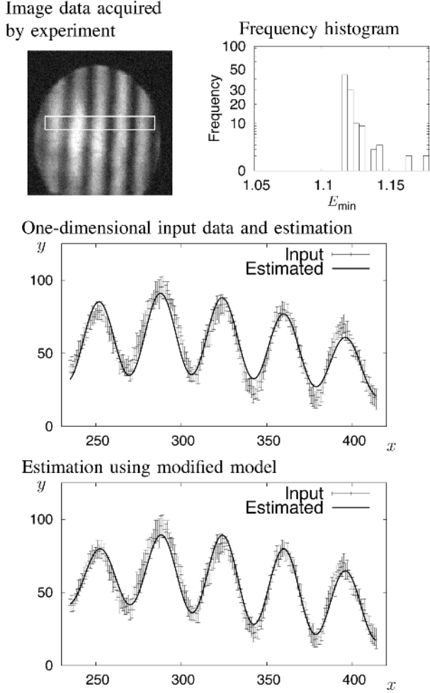
Fig. 10. Input data of “Exp” and its estimated result. The image data in left-top figure is obtained by an interferometer system with two light beams. The bounded area is used for the proposed estimation method. The input data for the proposed estimation method is prepared by computing the average and the standard deviation along the vertical axis for the every horizontal pixel. Both the input data and its estimated function obtained by the adaptive domain method of “ADM 4 GAs” are shown in the middle. The estimated function is of 50th rank in 100 trials. Each input data is plotted with an error bar that shows the standard deviation of the data itself. The top-right figure shows a frequency histogram of the least mean squares in 100 trials. The bottom figure shows the estimated result for modified model which assumes that the center and the width of two beams are different.
