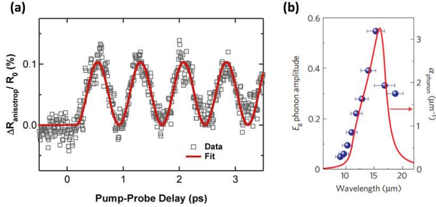
Fig. 3. (a) Time-resolved anisotropic reflectivity changes induced in \text{La}_{0.7}\text{Sr}_{0.3}\text{MnO}_3 by resonant excitation of the IR-active E_u stretching mode at 14\ \mu\text{m} . (b) Amplitude of the coherent E_g Raman oscillation (blue circles) and linear absorption coefficient (red line) of \text{La}_{0.7}\text{Sr}_{0.3}\text{MnO}_3 as function of pump wavelength. Panel (a) adapted from [43]. Panel (b) reprinted from [40].
