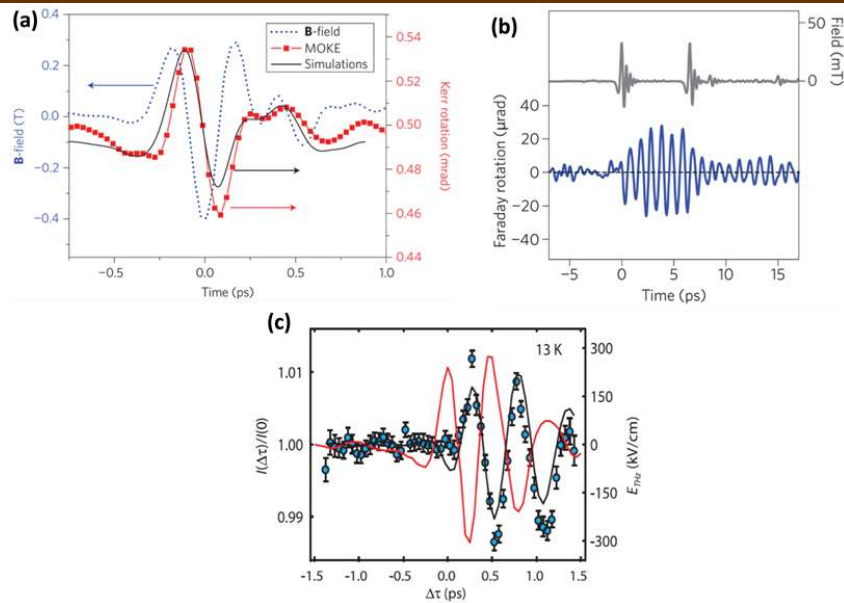
Fig. 23. (a) Femtosecond magnetization dynamics in 10-nm thick Co, represented by the MOKE signal (red curve) and initiated by single-cycle THz magnetic field (blue dotted curve). The black line indicates the simulated response [168]. (b) Magnetization dynamics (blue curve) measured in antiferromagnetic NiO after excitation with a pair of 0.5-ps, 40-mT THz transients (grey curve). The applied pulse sequence is shown to switch a 1-THz spin wave on and off [164]. (c) Magnetic diffraction intensity of the (0 q 0) peak of TbMnO 3 (blue symbols, left axis) compared with the electric field of the pump trace (red solid line, right axis) as a function of time delay, measured in the multiferroic phase ( T = 13 K) [172]. Panel (a) reprinted by permission from Macmillan Publishers Ltd: Nature Photonics [168], copyright 2013. Panel (b) reprinted by permission from Macmillan Publishers Ltd: Nature Photonics [27], copyright 2013. Panel (c) from [172]. Reprinted with permission from AAAS.
