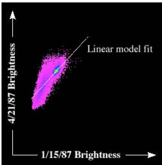
c) Joint distribution
