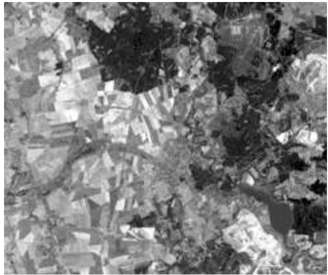
(b) Haze equalized band 1 image
