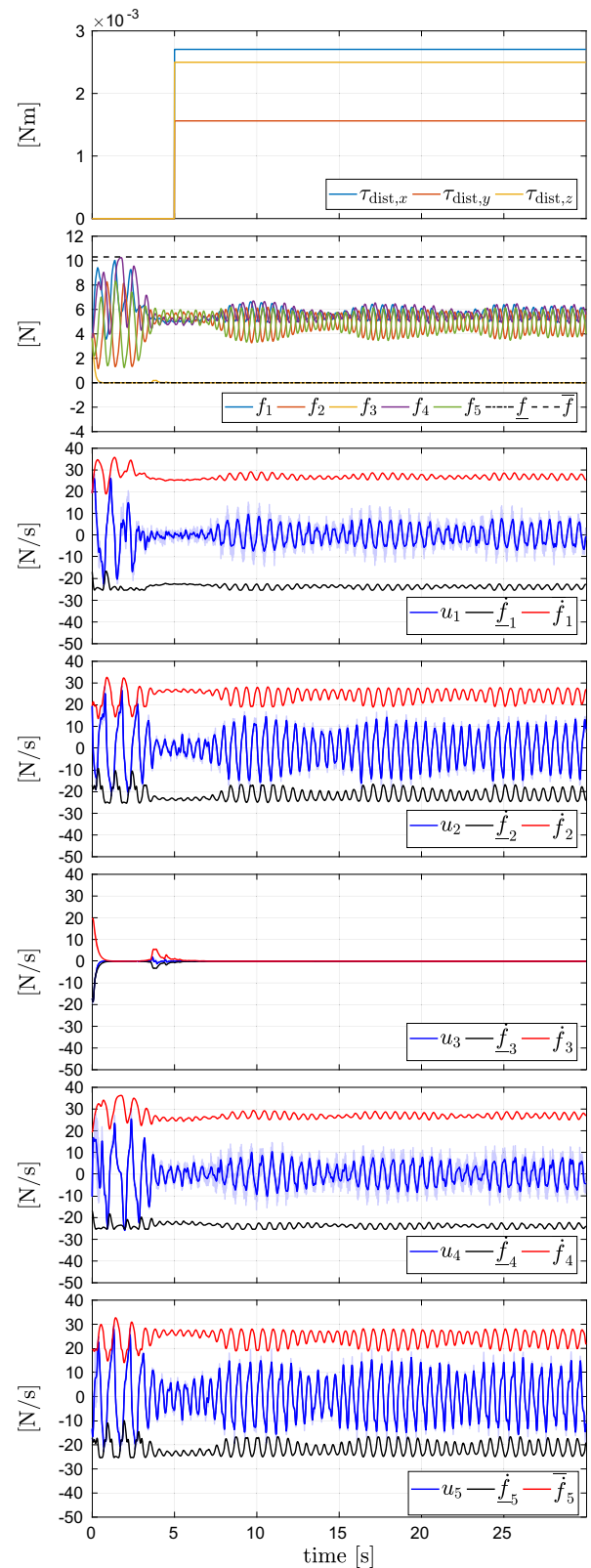
Fig. 21 Plots of the Tilt-Hex with rotor failure and \beta = 0 deg while hovering. The robot is disturbed with a constant external torque \tau_{dist} , activated at t = t_1 . From top to bottom, the disturbance torque, the actuator forces and their derivatives. In particular, all the signals remain inside the feasible region delimited by the constraints
