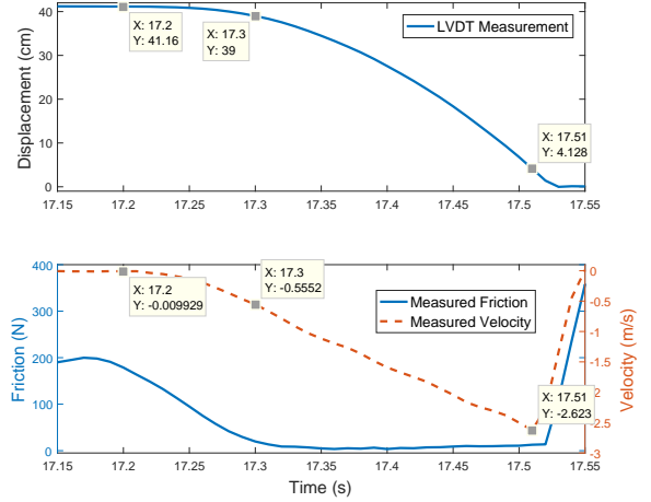
Fig. 6. Free-fall tests to determine the Coulomb and damping coefficients.
