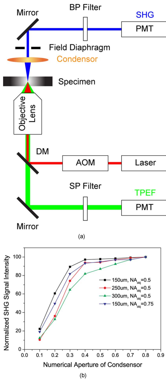
Fig. 1 (a) Schematic illustration of the optical configuration: Excitation laser was a tunable mode-locked laser (710–990 nm) with an AOM for power control. The laser went through a DM (490 nm), an objective lens, and reached tissue specimen. An SHG signal was collected on the opposite side the laser source, by a high NA condenser, through a field diaphragm and a 450-nm band-pass (BP) filter, before being recorded by a PMT. TPEF was collected by the objective lens, filtered by a 700-nm short-pass (SP) filter before being recorded by another PMT. (b) Dependence of SHG signal intensity on NA of the objective lens, NA of the condenser, and the thickness of liver slices. For thin tissue samples, thickness=150 μm, SHG signal intensity reached a plateau when NA of the condenser roughly equals to the NA of objective lens. However, for thick slices (~300 μm), SHG signal continued to increase even when the condenser NA is larger than the objective NA.
